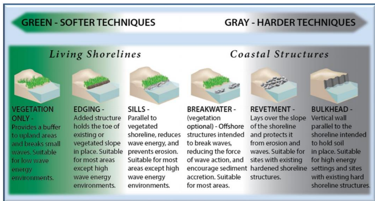
Figure 5.7. Continuum of shoreline stabilization methods, from most natural and softest (green) to least natural and hardest (gray), with the greenest methods being more effective in low to moderate wave energy, and grayest methods being more effective for high wave energy. 105
