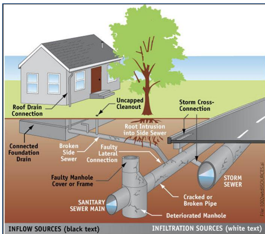
Figure 7.1. Example of inflow and infiltration (I & I) pathways. 2
