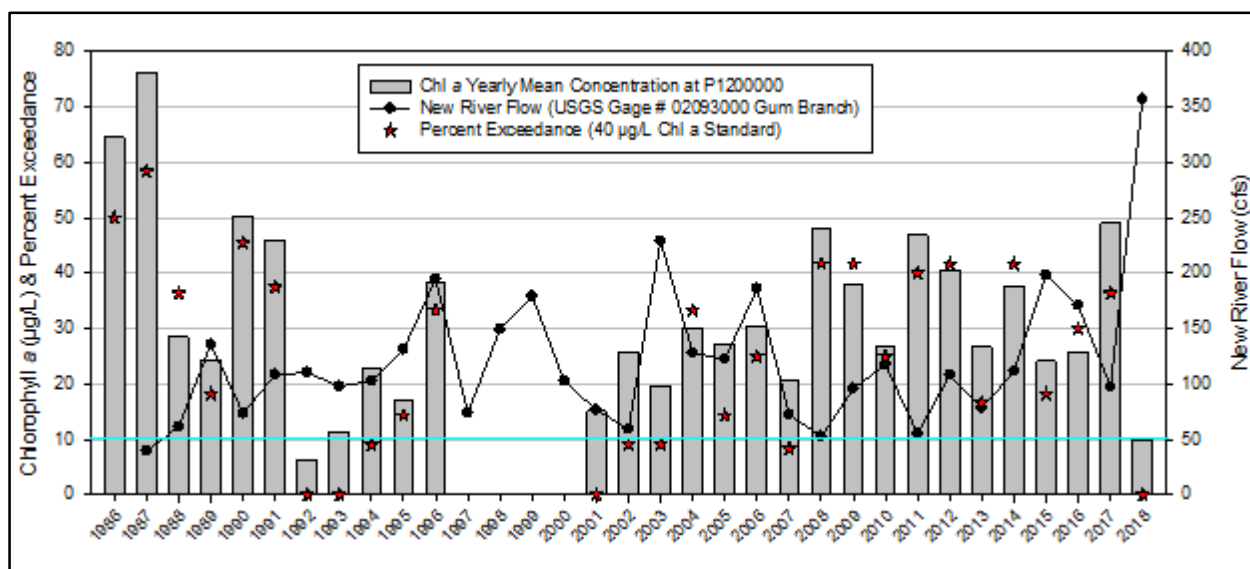
Figure. 8.13. Annual Mean Chlorophyll a Concentrations at the New River at Jacksonville US 17 Bridge Ambient Monitoring System (AMS) Station (P1200000) with Corresponding Percent Exceedance of the 40 µg/L Chlorophyll a Standard and Annual Mean New River Flow (blue line denotes the 10 percent excursion level).
