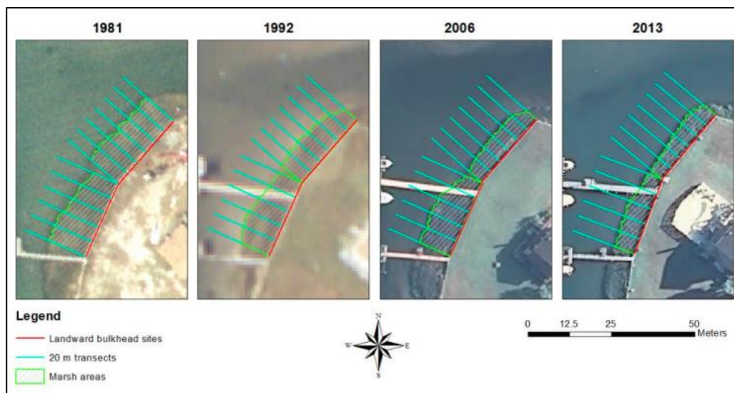
Figure 5.6. Time series of two bulkhead sites illustrating changes in marsh width, 1981-2013. 100
