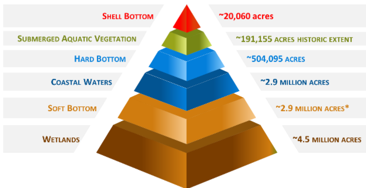
Figure 1.1. The coastal habitats of North Carolina are the foundation for healthy fisheries. *Soft Bottom habitat is an over estimation due to overlapping regions of the data used for analysis.
