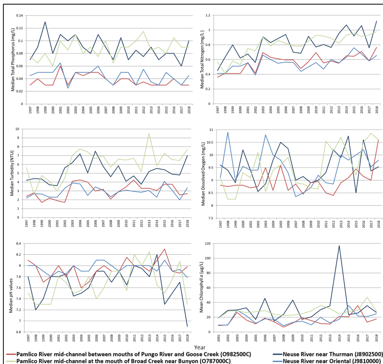
Figure 8.6. Annual median Total Phosphorus (mg/L), total Nitrogen (mg/L), Turbidity (NTU), DO (mg/L) concentrations, and pH values, and mean Chlorophyll a ( \mu g/L) concentrations for representative Ambient Monitoring System (AMS) stations in Coastal Habitat Protection Plan (CHPP) Region 2.
