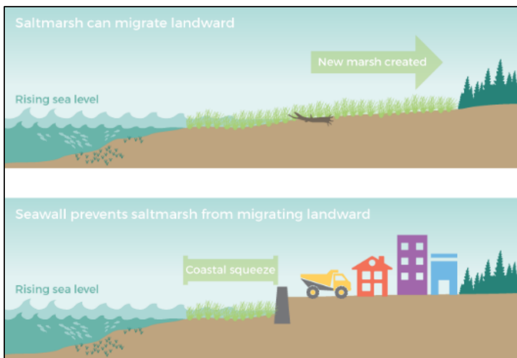
Figure 5.8. Conceptual diagram of process of natural marsh migration with sea level rise (SLR), and coastal squeeze when migration is impeded.
