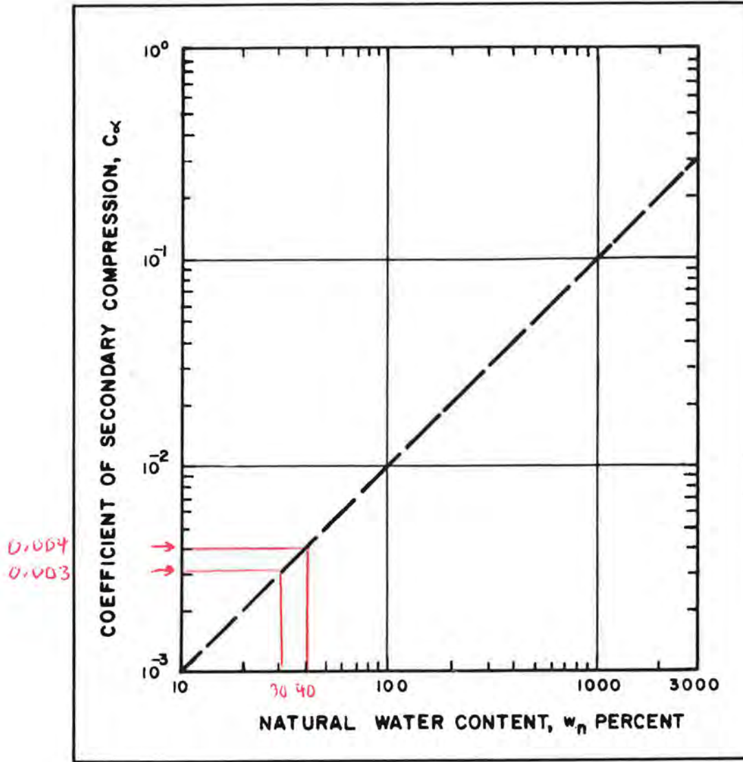
FIGURE 16 Coefficient of Secondary Compression as Related to Natural Water Content
