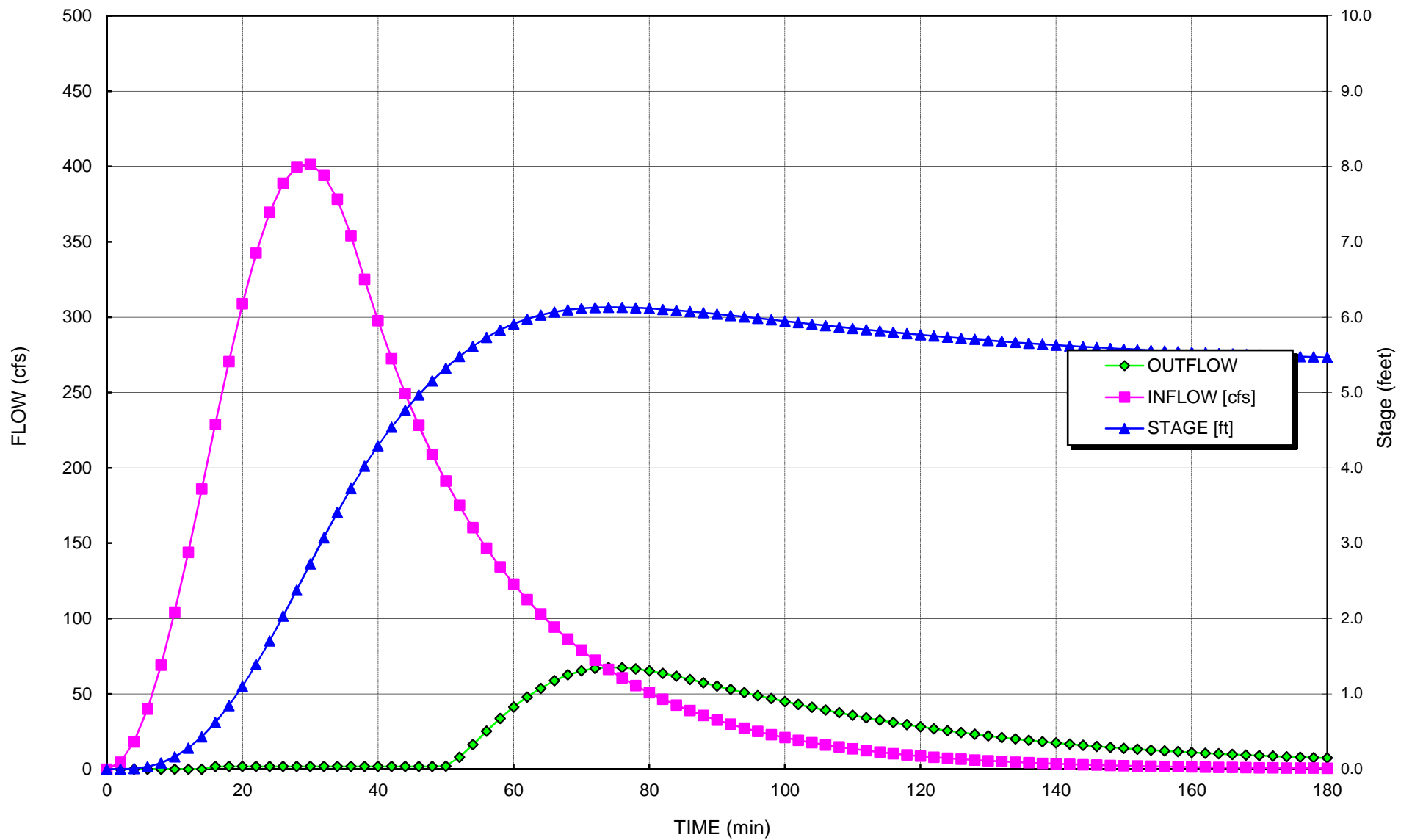
Sediment Basin #5 Colon Mine Phase 2 Hydrograph 100-Yr Storm
