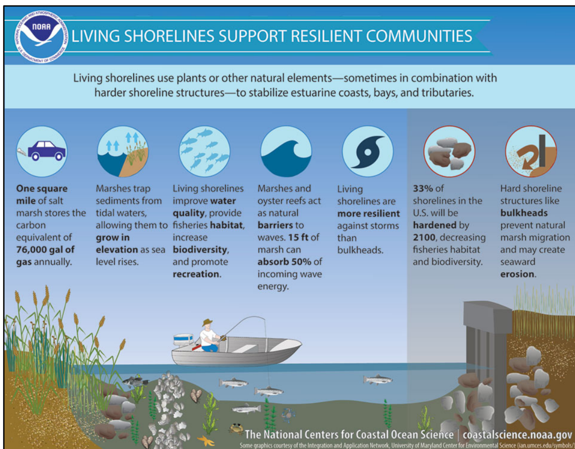
Figure 2.5. The ecosystem benefits of living shorelines for shoreline stabilization.
