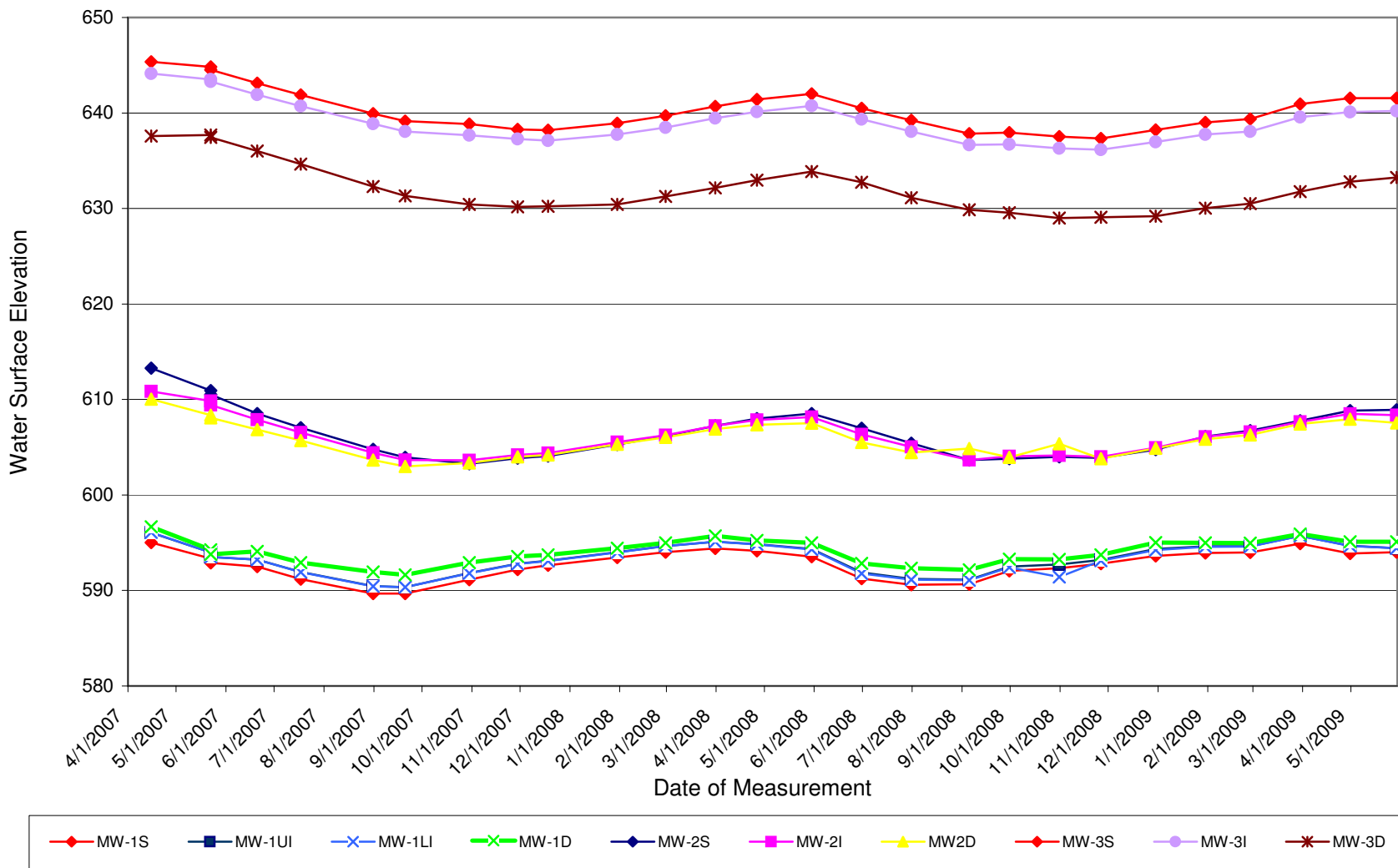
Figure 3. Groundwater Levels at NC Zoo Groundwater Monitoring and Research Station
