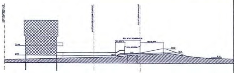
230 CAROLINA BEACH AVE. NORTH LONGITUDINAL SECTION SCALE: 1/8" = 1'-0" NOTE: FINAL REVISION: LOWERS THE PROPOSED BOARDWALK FROM 10.0 TO 10.0 WHICH SHORTENS RAMP, REQUIRES LESS STEPS. ALL POLE LIGHT FIXTURES ARE REMOVED ON NORTHERN EXTENSION
