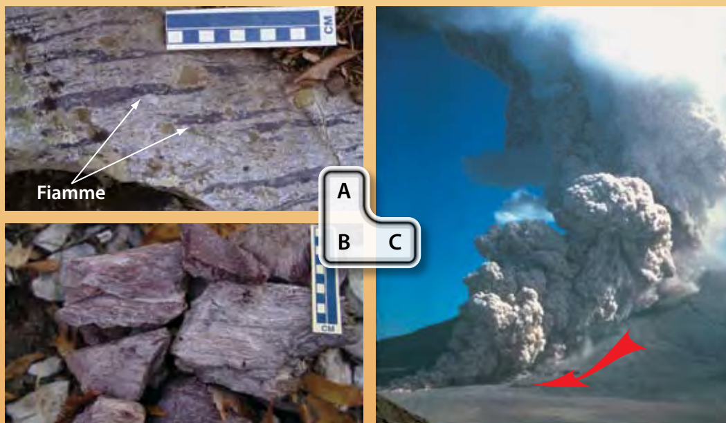
Figure 9 – Examples of ancient and modern day pyroclastic flow deposits.
