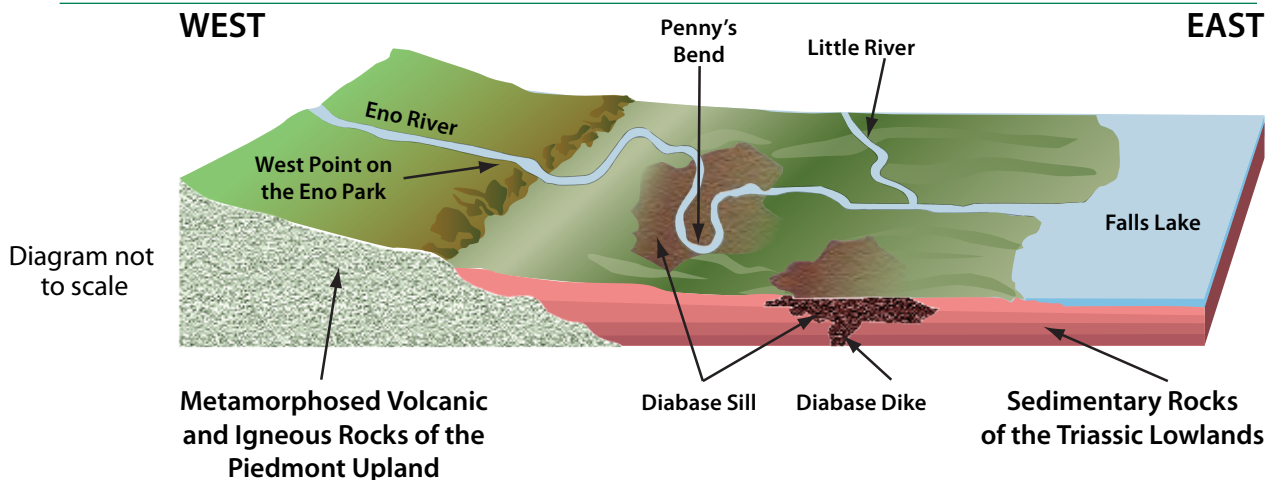
Figure 3 - 3-D generalized diagram of the Eno River as it flows over the boundary of the Piedmont upland and Triassic lowland.
