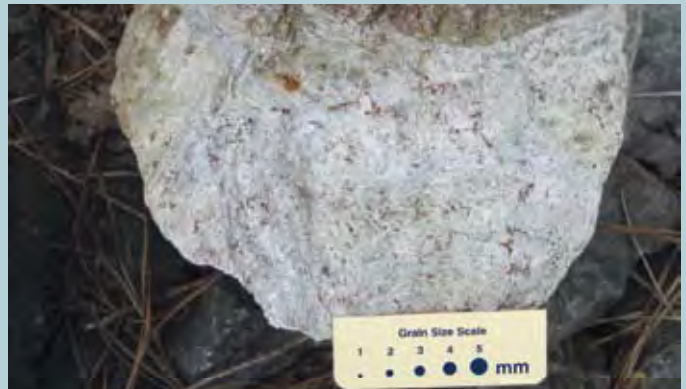
Figure 47 - Example of light gray to white, hydrothermally altered tuff from the former Eno Quarry.
