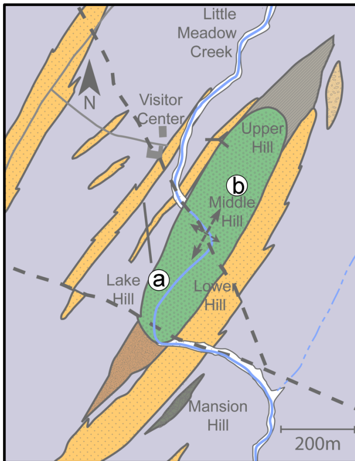
Figure 11: Locales for geochemical sampling at the RGM. Samples for whole rock elemental analysis were collected at site a on Lake Hill and site b on Middle Hill. Zircons for dating were separated from samples collected at site a.
