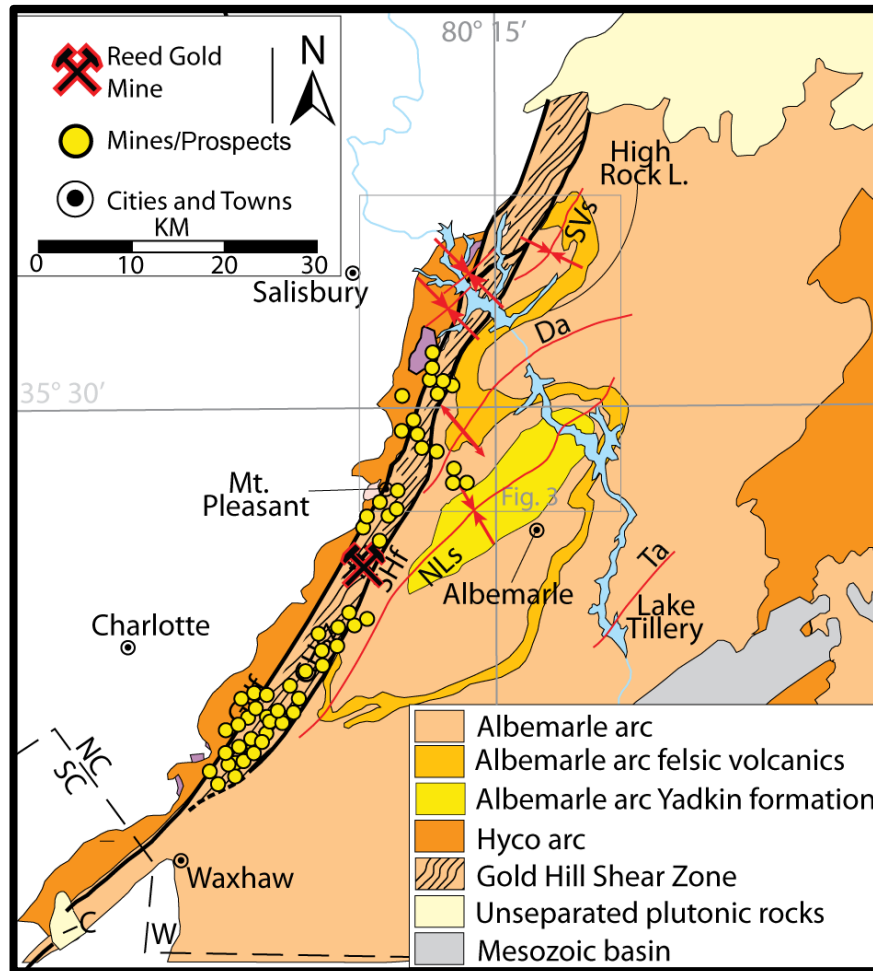
Figure 2: The RGM is located in the GHsz, along the boundary between the Albemarle and Hyco arcs. The GHsz is the site of numerous historical gold mines and prospects; approximate locations of selected regional mines and prospects from Nitze and Hanna (1896). Most of the regional folds associated with the GHsz, are noncylindrical. One notable example is the New London Syncline (NLS); the outcrop pattern of the Albemarle arc felsic volcanics and the Yadkin Formation clearly show that it is doubly plunging (adapted from Pollock and Hibbard, 2010; Hibbard et al., 2012).
