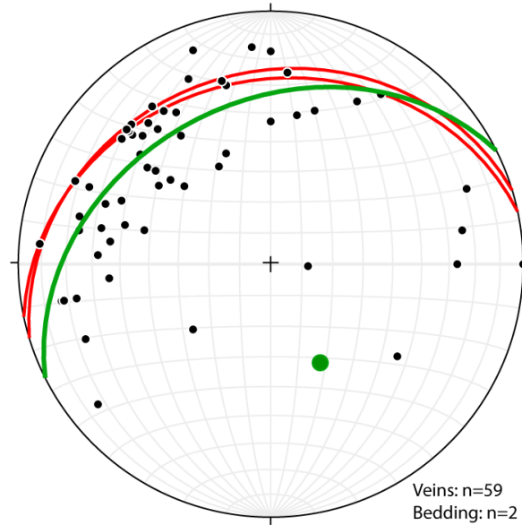
Figure 20: Poles to quartz veins measured in the underground workings define a great circle (marked in green). The great circle defined by poles to veins is subparallel to bedding measurements taken in immediately adjacent sediments (marked in red, based on data from El-Samani (1978)).
