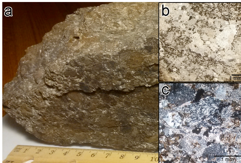
Figure 9: At first glance, the feldspar clasts give the volcaniclastic conglomerate a porphyritic appearance. On closer inspection, however, the rock is composed of diverse angular to rounded volcanic clasts. (b) At 40x a variety of clasts can be seen. Although many clasts are largely altered, some feldspars are largely intact and some clasts preserve original volcanic textures. (c) A prominent clast with trachytic texture viewed at 100x with crossed polars.
