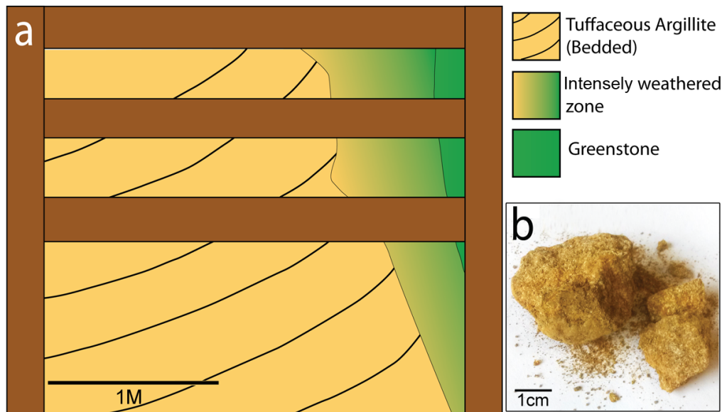
Figure 16: (a) Schematic view of the contact between tuffaceous argillite and the RGM gabbro in the wall of Linker adit, with the rock visible between wooden slats (in brown). The image is constructed from photos taken during the course of underground mapping. Bedding in the argillite deflects upward as it approaches the contact. Within the heavily weathered zone around the contact primary texture and sedimentary features are almost entirely obscured and both rock types are a light tan color; as such the two are difficult to distinguish. The gabbro adjacent to the contact (b) is saprolitic and can easily be crumbled into silt- and clay-sized particles.
