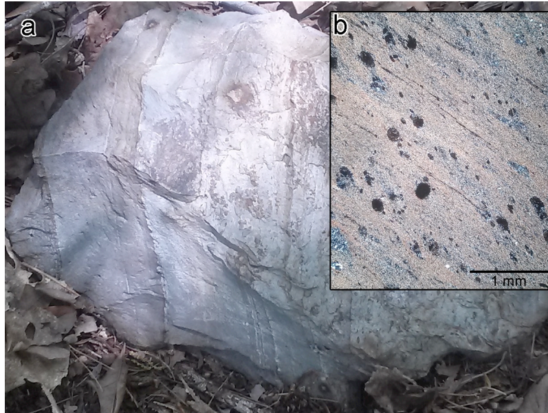
Figure 7: Slaty Argillite. A typical hand sample (a) is fine grained aside from large pyrite cubes, and displays pronounced cleavage. Bedding features are readily observed. In thin section view (b) parallel extinction, fine lines of dark red oxidized biotite and irregular blobs of leucoxene are observed.
