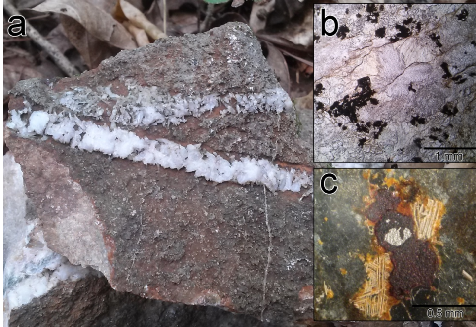
Figure 10: RGM gabbro. Hand sample approximately 15 cm across in (a), featuring two quartz veins. In (b), at 20x with uncrossed polars, extensive chloritization and skeletal black opaques are visible. In (c) a reflected light image at 40x reveals detail within the opaques. The skeletal white opaques are likely leucoxene, the red likely limonite after pyrite, and the metallic blebs within the red are likely gold.
