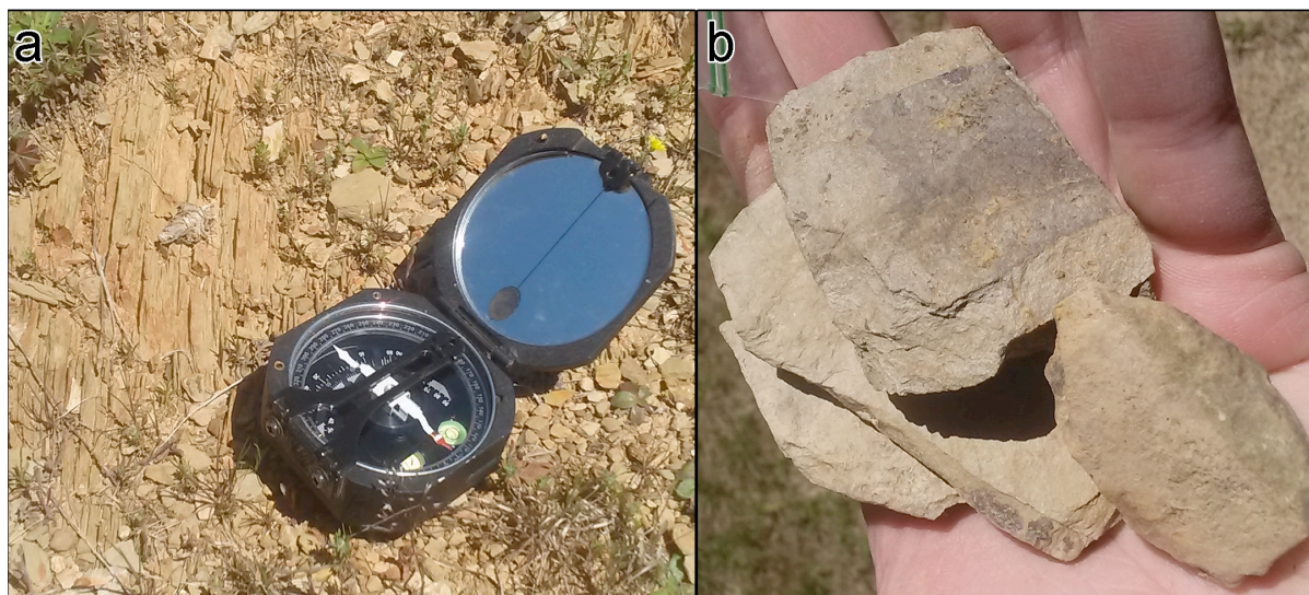
Figure 5: A typical outcrop of laminated argillite (a) along with cleavage flakes (b). Main access road to the Reed Gold Mine state historic site.
