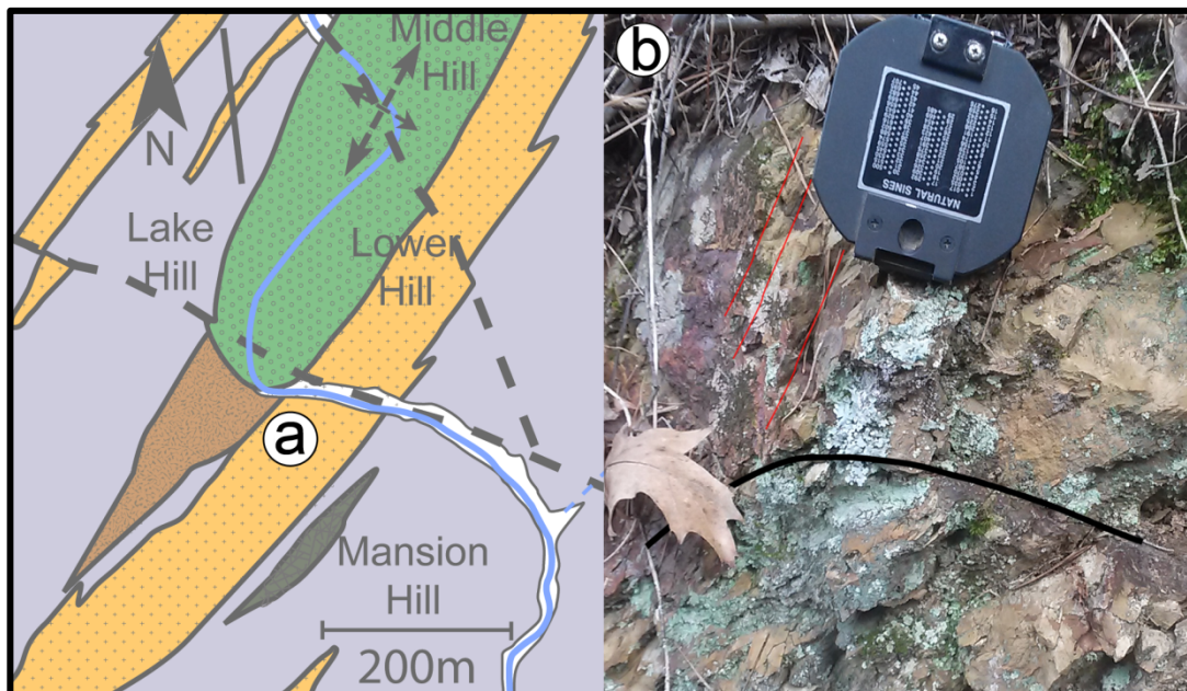
Figure 18: At site (a) on the map, a small southwest-plunging fold was observed in an outcrop (b). Cleavage traces marked in red on (b) are axial planar to the fold, showing that it is parasitic to the main RGM fold.
