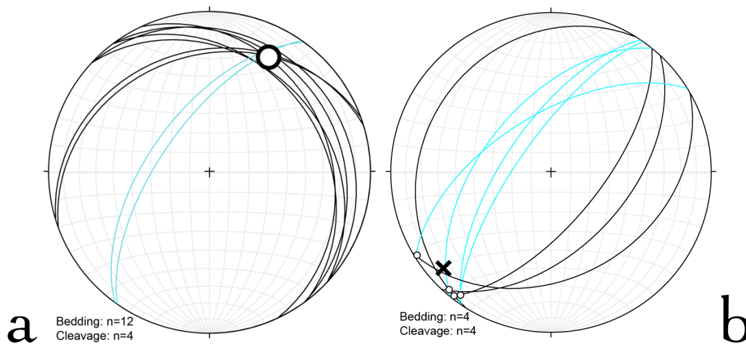
Figure 17: a. The line of intersection of bedding and cleavage orientations from stratified rocks in the northeastern area of the RGM property plunges to the northeast, indicating a northeast plunge to the fold in that area. b. Four pairs of bedding orientations (in black) and cleavage orientations (in blue) from the southwestern portion of the RGM from the present study and El-Samani (1978). The line of intersection between each bedding and cleavage pair (marked with white circles) plunges shallowly to the southwest, indicating that the fold plunges to the southwest in this area. The axis of a single parasitic fold measured in the same area, marked with an X, plots close to the intersections.
