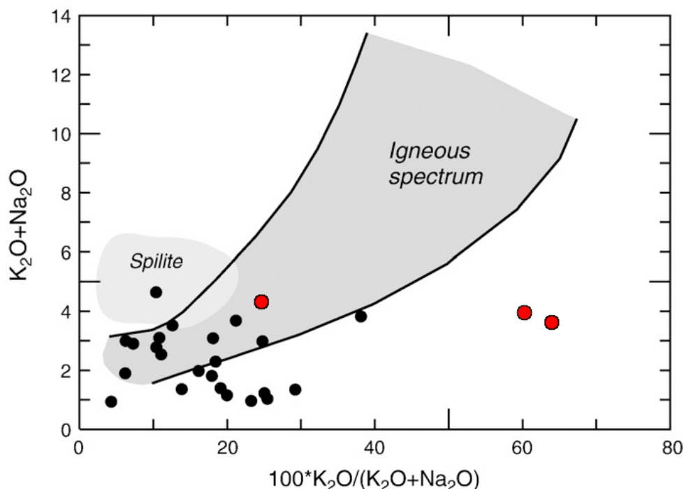
Figure 13: RGM gabbro samples from Lake Hill (fig. 11a) plot outside the igneous spectrum (Hughes, 1972), indicating mobilization of K and Na after the initial intrusion. The sample from Middle Hill (Fig. 11b) is within the igneous spectrum with values similar to members of the SMis, indicating that mobilization was related to local alteration rather than regional metamorphism (adapted from Pollock and Hibbard, 2009, Fig. 6).
