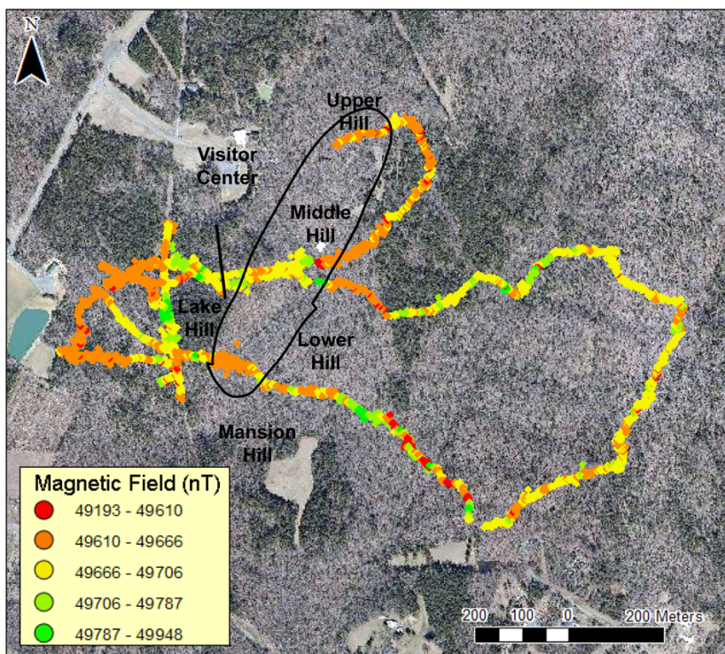
Figure 19: Geomagnetometric data collected at the RGM, plotted over a 2015 orthophoto of the area (NC Onemap, 2015) with the outcrop pattern of the RGM gabbro superimposed over it. After processing and despiking, numerous small anomalies are visible with a broad trend towards lower values in the eastern area of the property. If the RGM gabbro had intruded as a vertical dike a relatively strong magnetic signal would be expected with a sharp magnetic drop off on either side.
