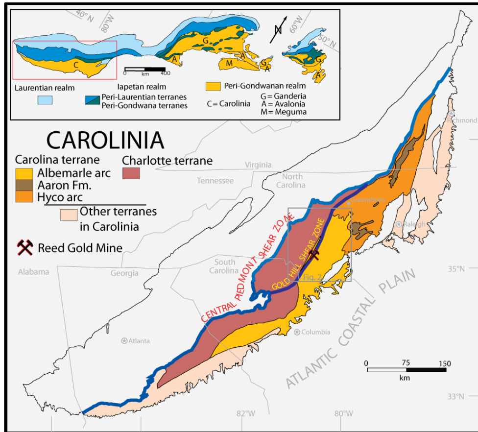
Figure 1: The Reed Gold Mine is centrally located in Carolina, in the Gold Hill shear zone, near the western edge of the Carolina terrane (adapted from Hibbard et al., 2006, 2012).
