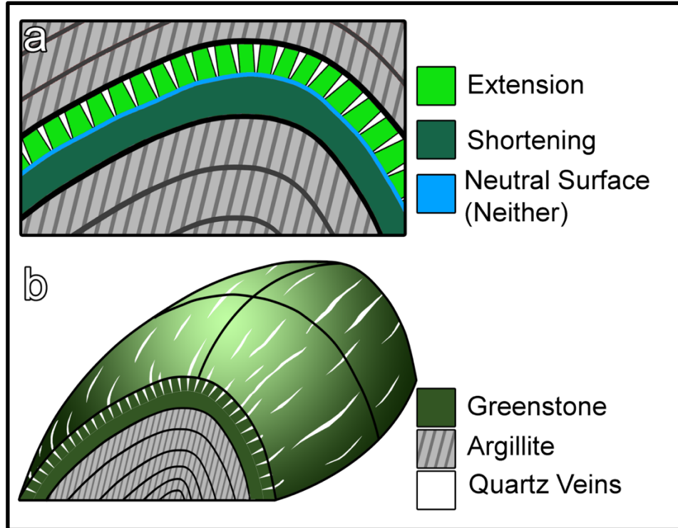
Figure 21: Visualization of the folded sill model for the RGM gabbro, shown in shades of green. In (a) zones of extension and shortening, and the neutral surface that experiences neither, are marked. Extension is accommodated by fractures that host auriferous quartz veins. In (b) a three-dimensional rendering shows the two fold axes in black that define the doubly plunging fold. White quartz veins are orthogonal to the tighter northeast-trending fold. In (a) and (b) parallel grey lines denote axial planar cleavage.
