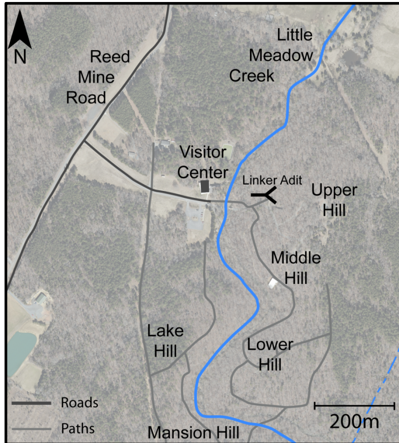
Figure 3: The RGM mine site, with major roads, paths and landmarks overlaid on a 2015 orthophoto of the area (NC OneMap, 2015).
