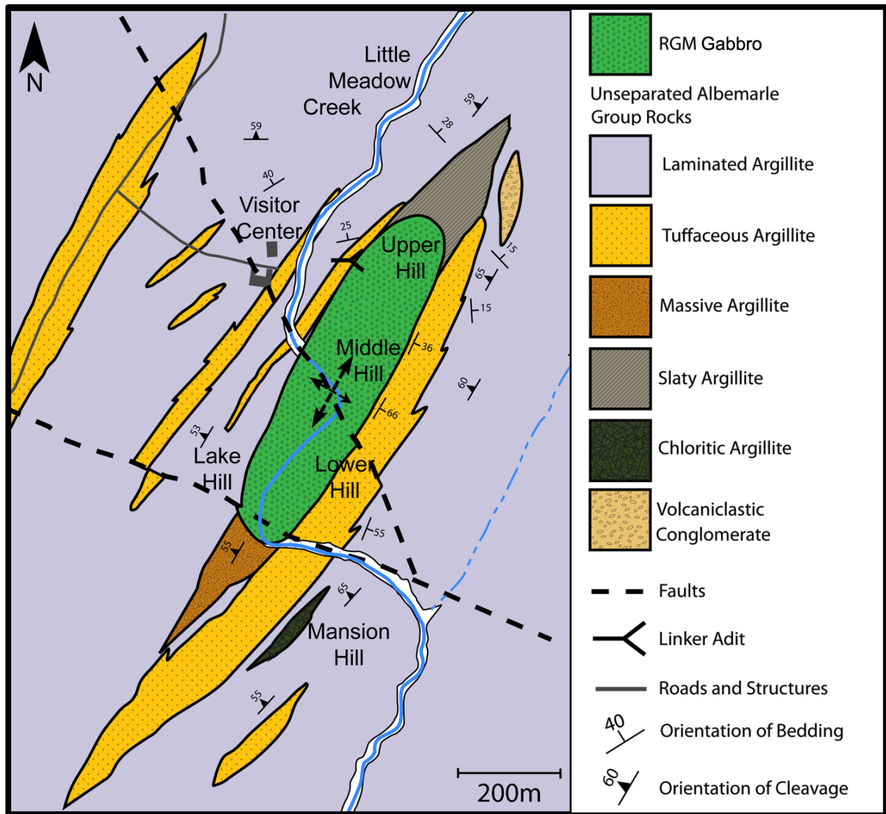
Figure 4: Geological map of the RGM based on observations made during the present study; where there was no conflict with map data from this study, contacts were adapted from El-Samani (1978). Selected orientations of bedding and cleavage come from measurements made during this study as well as those compiled from El-Samani (1978).
