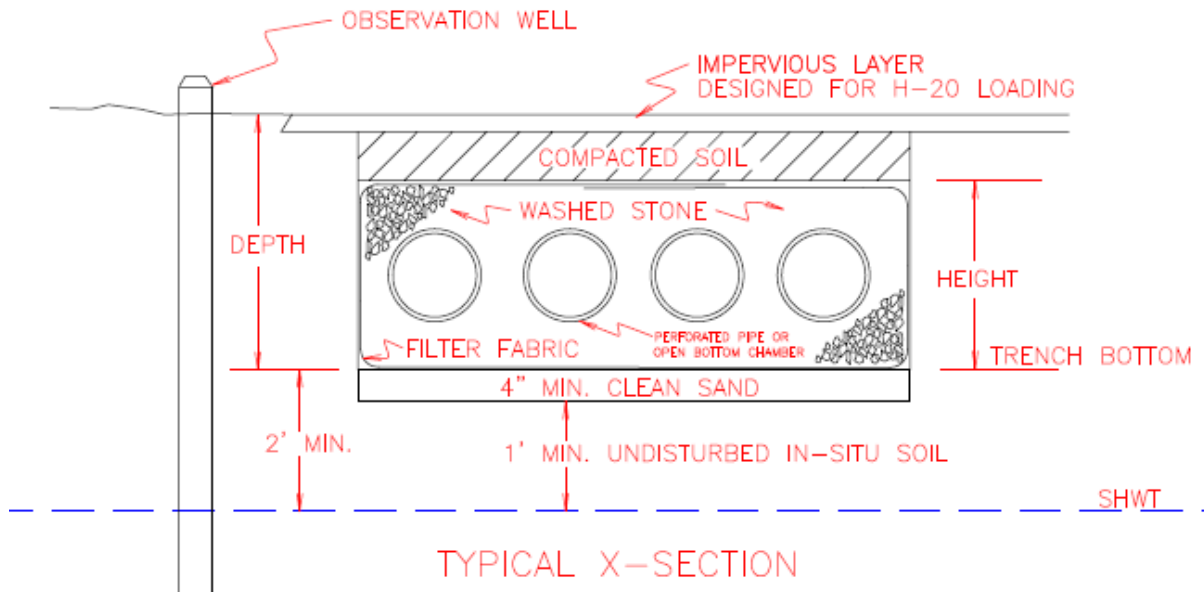
Figure 16-1b Typical Infiltration Trench: Cross-Section
