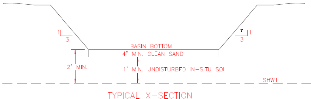
Figure 16-2 Typical Infiltration Basin: Cross-Section
