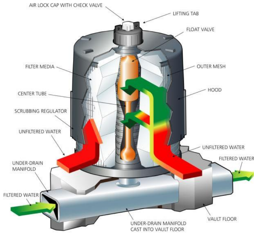
Figure 1: StormFilter Cartridge
