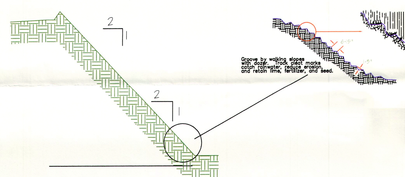
Typical Fill Slope Details
