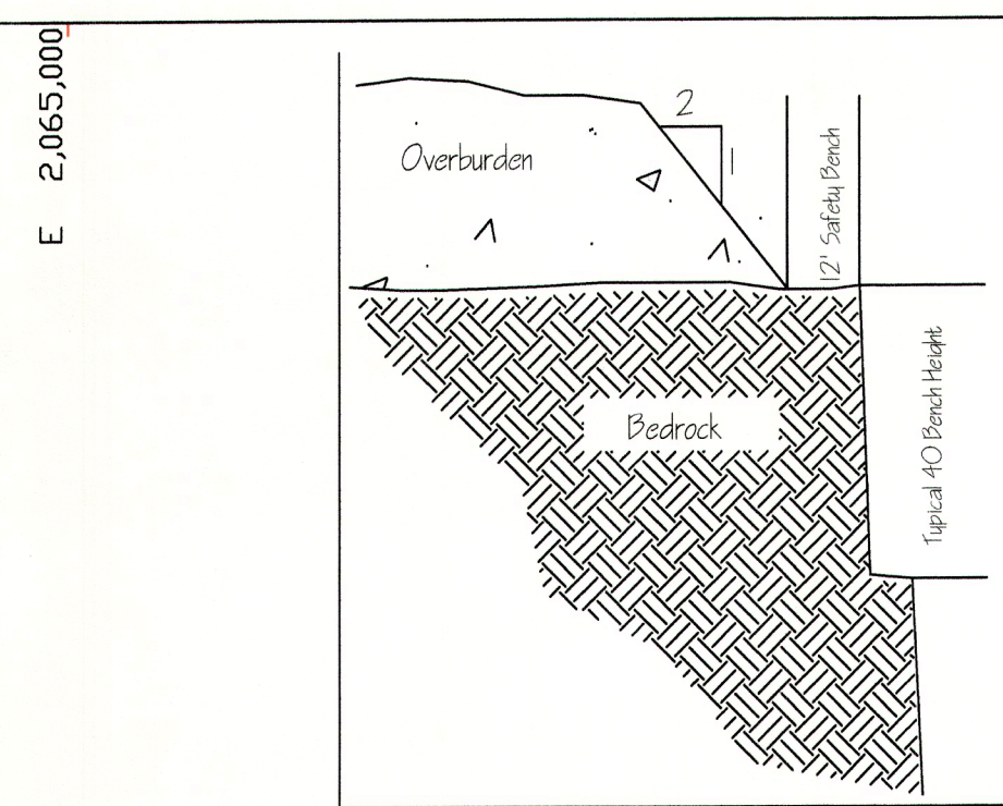
Typical Overburden Cut Slope and Pit Bench Details
