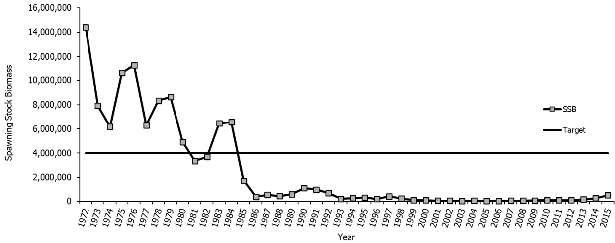
Figure 1. Annual predicted spawning stock biomass (SSB) in pounds for the Chowan River blueback herring stock, compared to the SSBTarget, 1972–2015. SSB is a stock status indicator and 2015 is the terminal year for the last river herring stock assessment update (ASMFC 2017).
