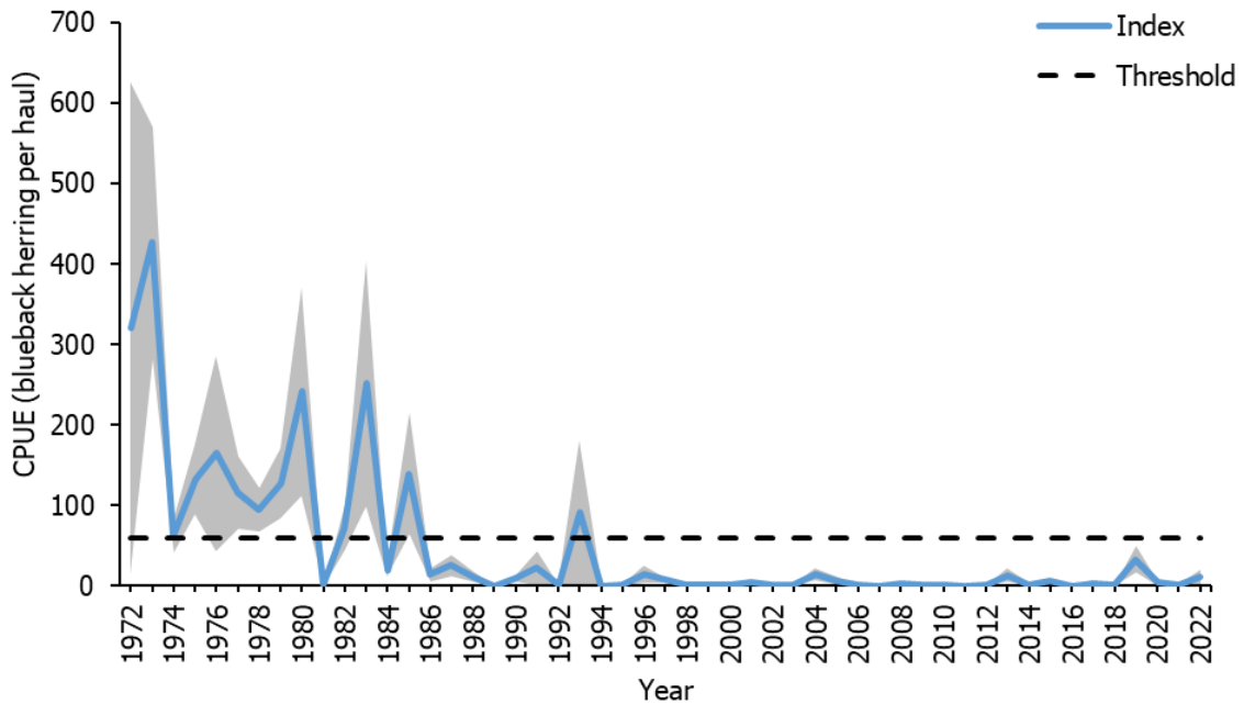
Figure 6. Catch per unit effort (fish per haul) and target of blueback herring collected from Program 100 in Albemarle Sound during June through October 1972–2022. Error bars represent \pm 1 standard error. Blueback herring relative abundance is a stock status indicator.
