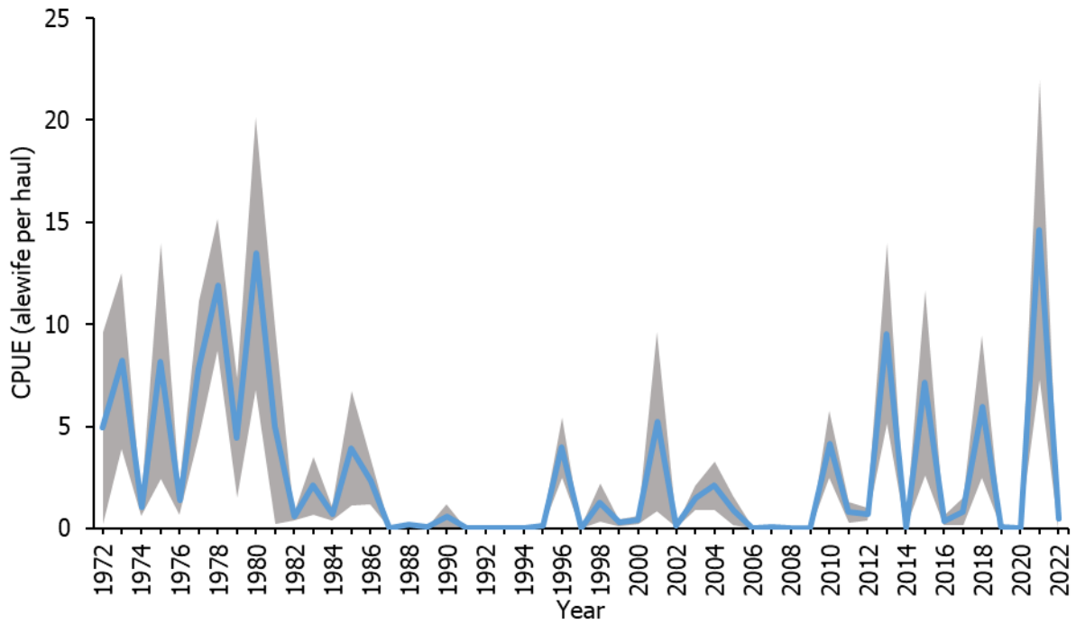
Figure 7. Catch per unit effort (fish per haul) of alewife collected from Program 100 in Albemarle Sound during June through October 1972–2022. Error bars represent \pm 1 standard error.
