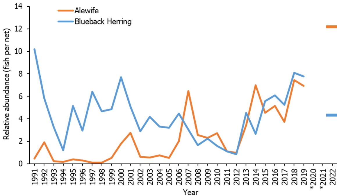
Figure 8. Relative abundance index of river herring (fish per net, 2.5- and 3.0-inch stretch mesh only) collected from Program 135 in Albemarle Sound during January through May 1991–2022. * Survey suspended February 20, 2020 and did not resume until fall 2021.
