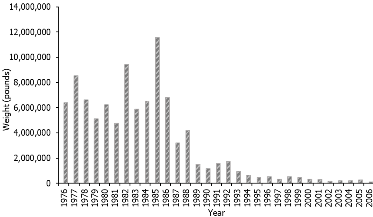
Figure 2. Commercial harvest (weight in pounds) of river herring from North Carolina, 1972–2006. Commercial harvest prohibited since 2007.
