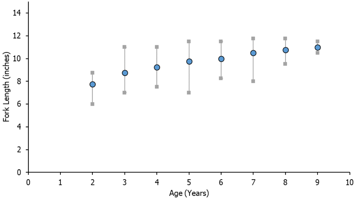
Figure 3. Blueback herring length at age from all age samples collected from fishery-dependent monitoring, 1972–2021. Blue circles represent the mean size at a given age while the grey squares represent the minimum and maximum observed size for each age. Age data from 2022 is unavailable.
