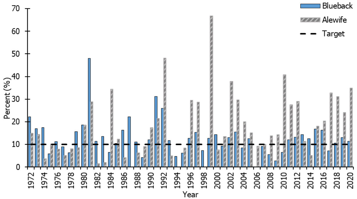
Figure 5. Annual percent of repeat spawners (blueback herring and alewife) and target from the Chowan River Pound Net Survey, 1972–2021. Blueback herring percent repeat spawner is a stock status indicator. Repeat spawner data from 2022 is unavailable.
