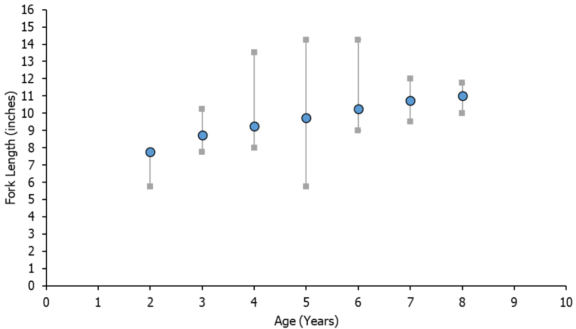
Figure 10. Alewife length at age from all age samples collected from Program 135 in the Albemarle Sound, 1972–2021. Blue circles represent the mean size at a given age while the grey squares represent the minimum and maximum observed size for each age. * Survey suspended February 20, 2020, and did not resume until fall 2021. Age data from 2022 is unavailable.
