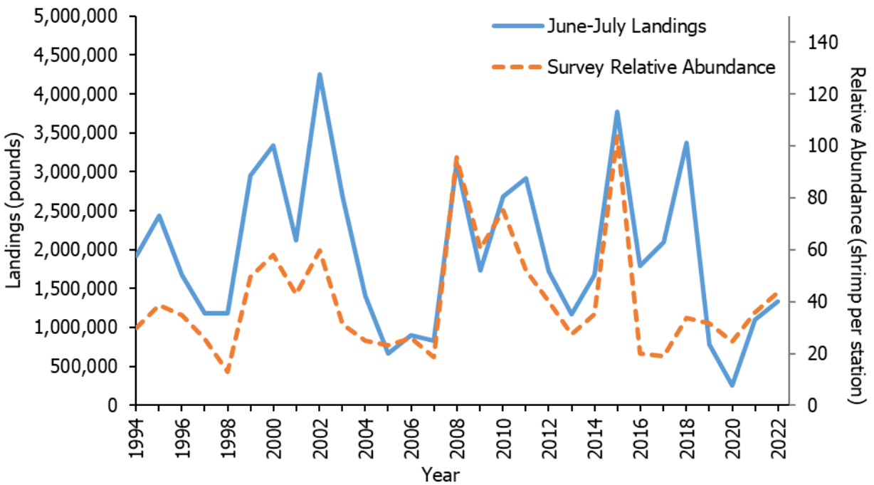
Figure 6. Comparison of brown shrimp commercial shrimp landings (pounds) in the months of June and July to the brown shrimp Program 120 index of relative abundance (shrimp per station), 1994-2022.
