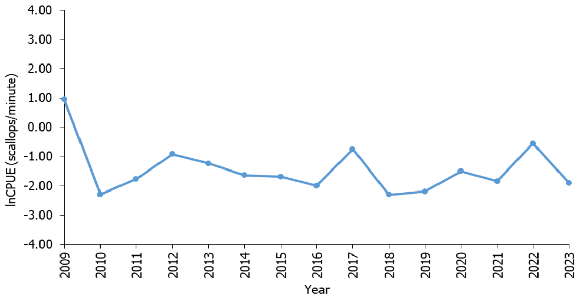
Figure 3. The mean number of bay scallops (lnCPUE) (bay scallops/minute) for areas south of Bogue Sound in October 2009–2023. Target opening estimates and progressive triggers will not be defined for this region until sampling is expanded and a longer time series is established.
