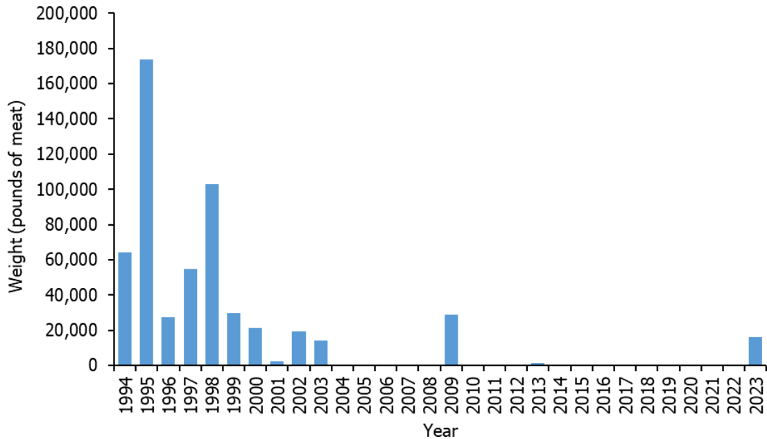
Figure 4. Bay scallop landings (wild and aquaculture in pounds of meat) in North Carolina, 1994–2023. Landings occurred in 2010, 2013, 2019, 2020, and 2022 but are not evident in the figure due to the scale required to show the range of landings for the time series.
