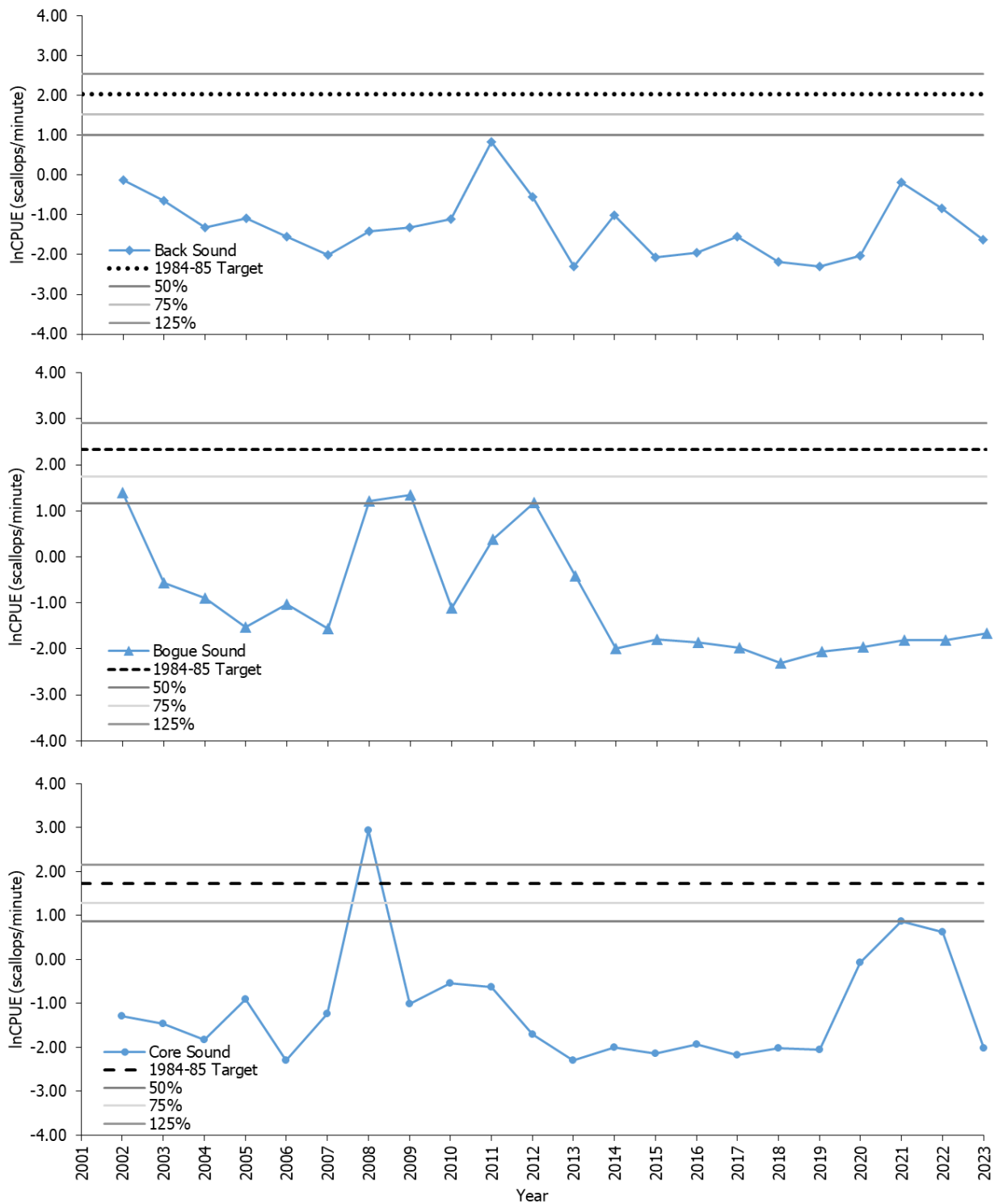
Figure 1. The mean number of bay scallops (InCPUE; bay scallops/minute) for Back, Bogue, and Core sounds during the October-December sampling time-period and average InCPUE (target) for the 1984–1985 period showing progressive triggers at 50, 75, and 125% of the target. Year indicates the sampling year which is used to determine the harvest season for the next calendar year.
