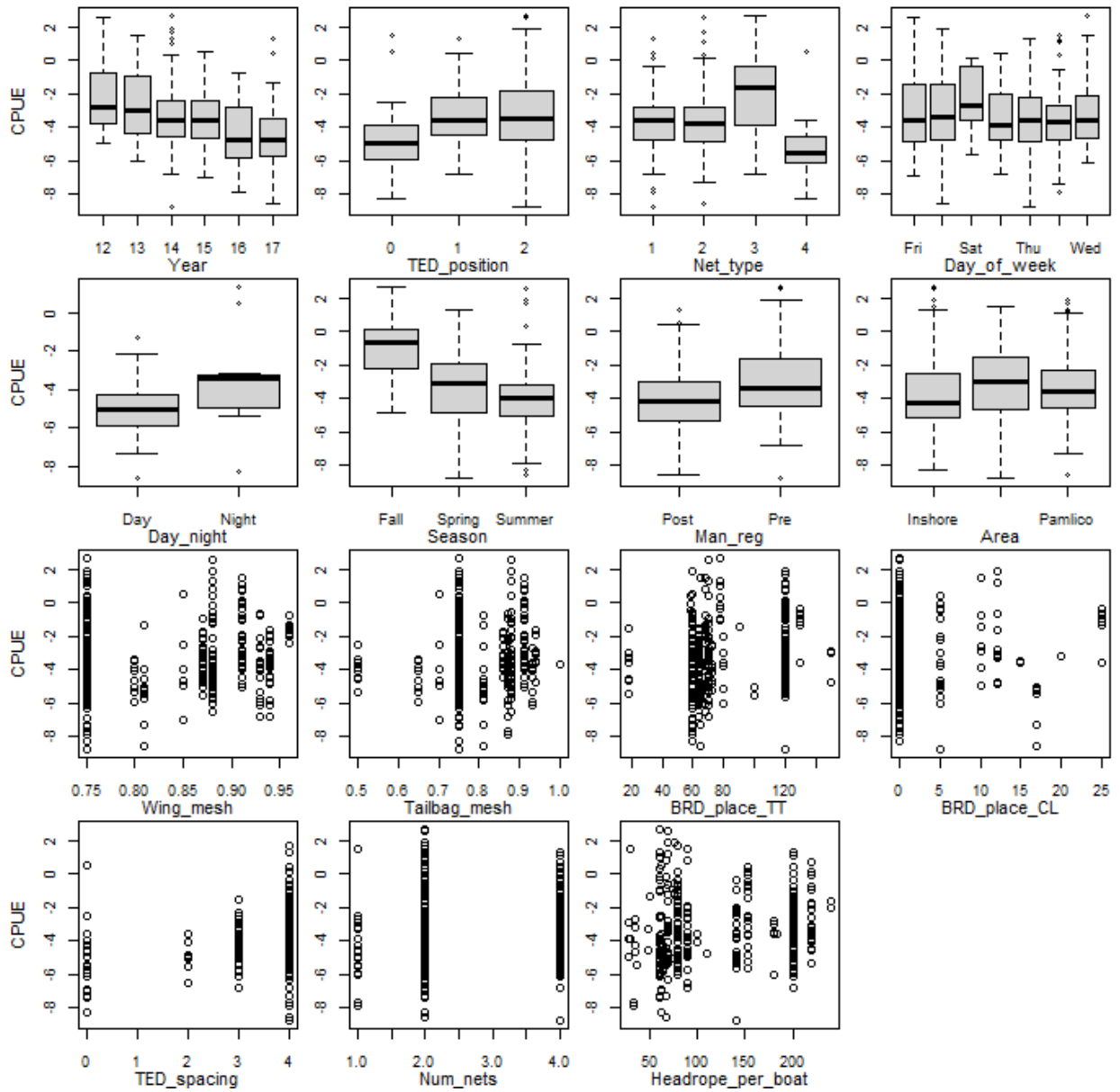
Figure 2.4.A.18. Plots of \log(\text{CPUE}) against each potential predictor variable for southern flounder.
