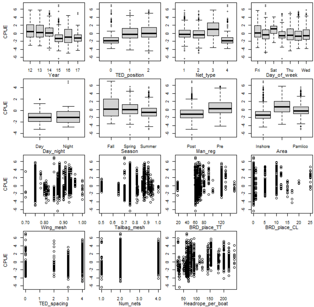
Figure 2.4.A.10. Plots of log(CPUE) against each potential predictor variable for finfish.
