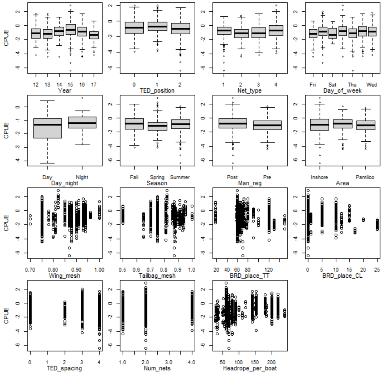
Figure 2.4.A.13. Plots of \log(\text{CPUE}) against each potential predictor variable for key shrimp (brown, white, and pink).
