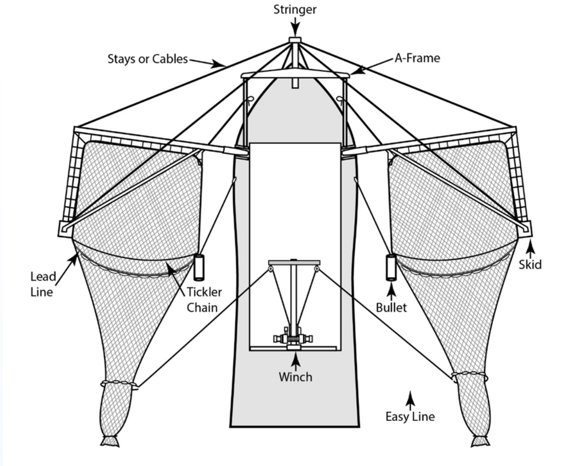
Figure 4. Schematic of skimmer trawler components.
