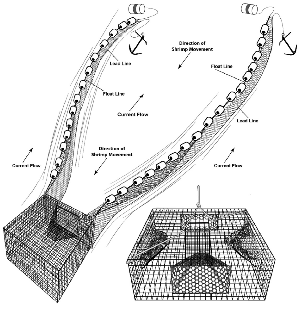
Figure 6. Schematic of a shrimp pound (A) and shrimp pot (B) components.
