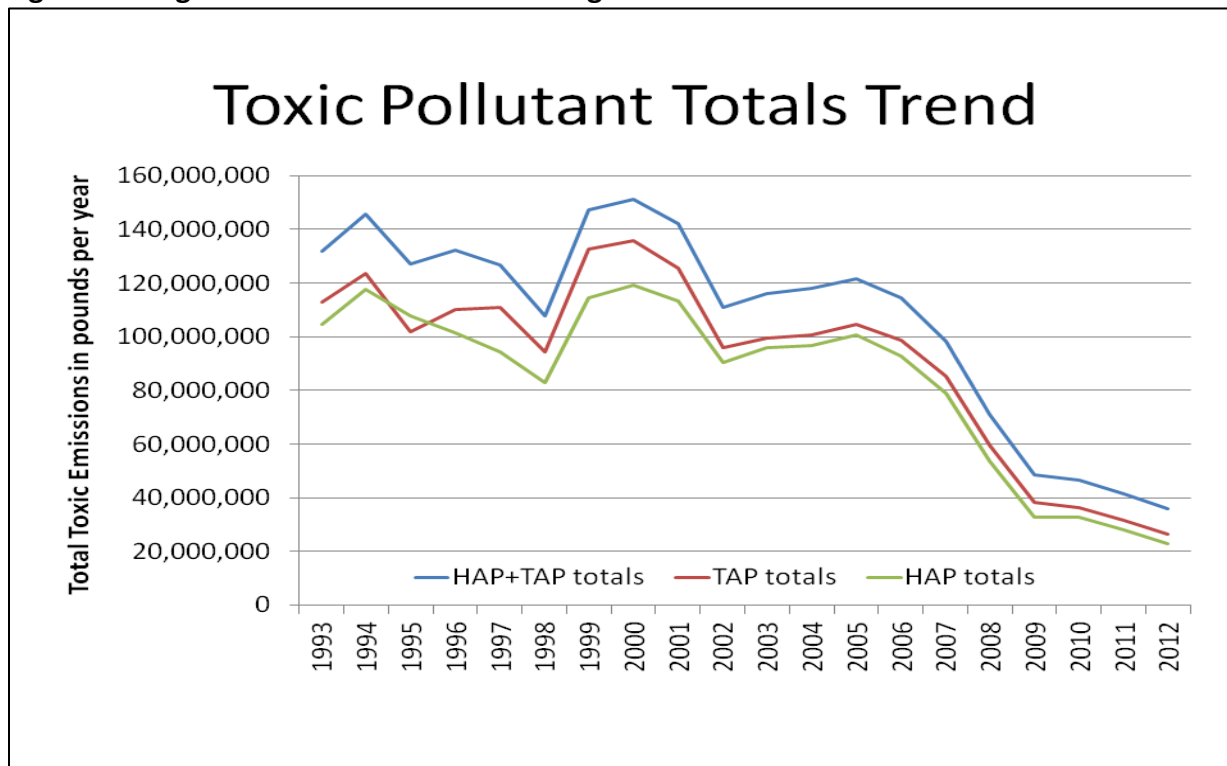
Figure 1. Long-term air toxic emissions changes 1993-2012
