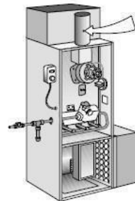
80+ Induced-draft Furnace
