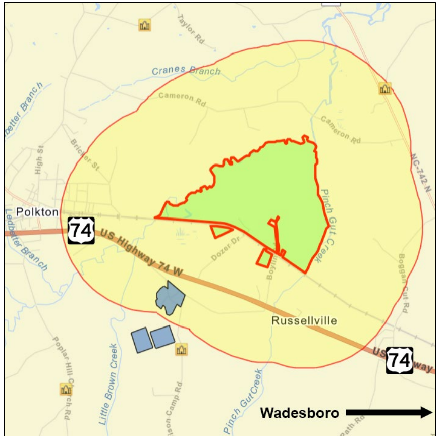
Anson Gas Producers, LLC footprint (approx.) in green with a 1-mile buffer around the facility.
