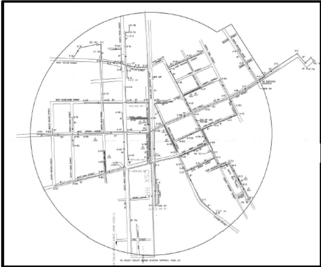
Figure 3 – Whitakers Sanitary Sewer Collection System Sizes and Location
