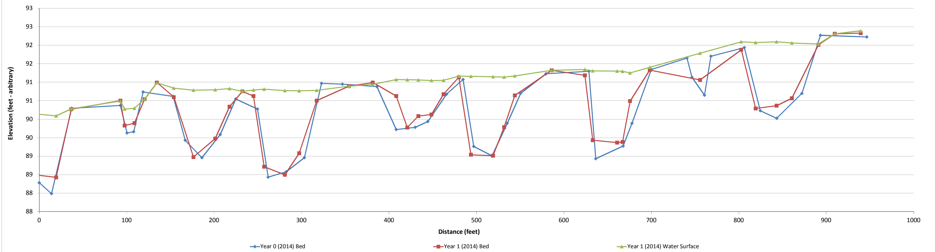
Bear Creek Year 1 (2014) Profile - Reach 2 (Downstream), Station 00+00 to 10+00
