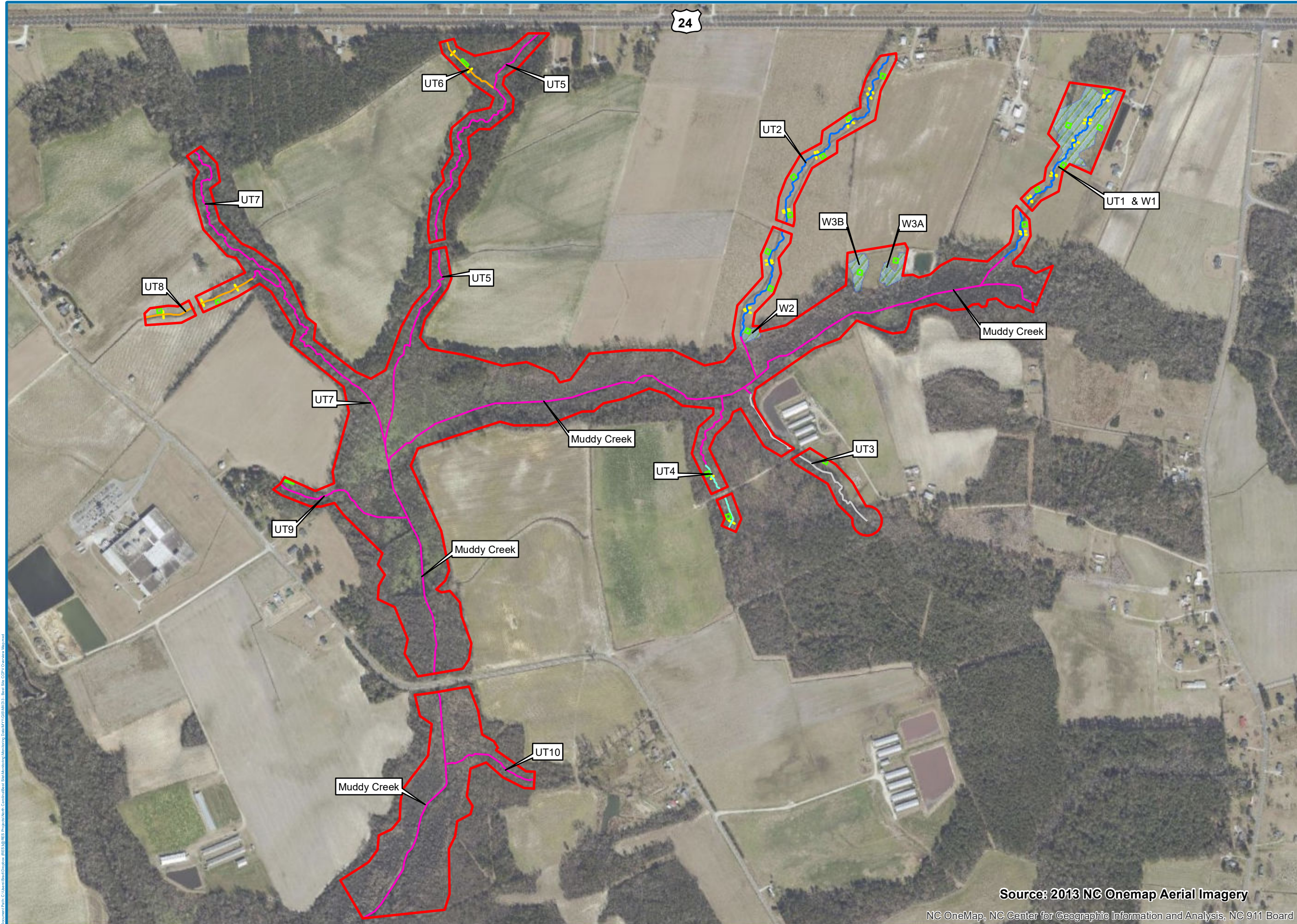
Figure 3. Best Stream and Wetland Restoration Project Current Conditions Overview Map
