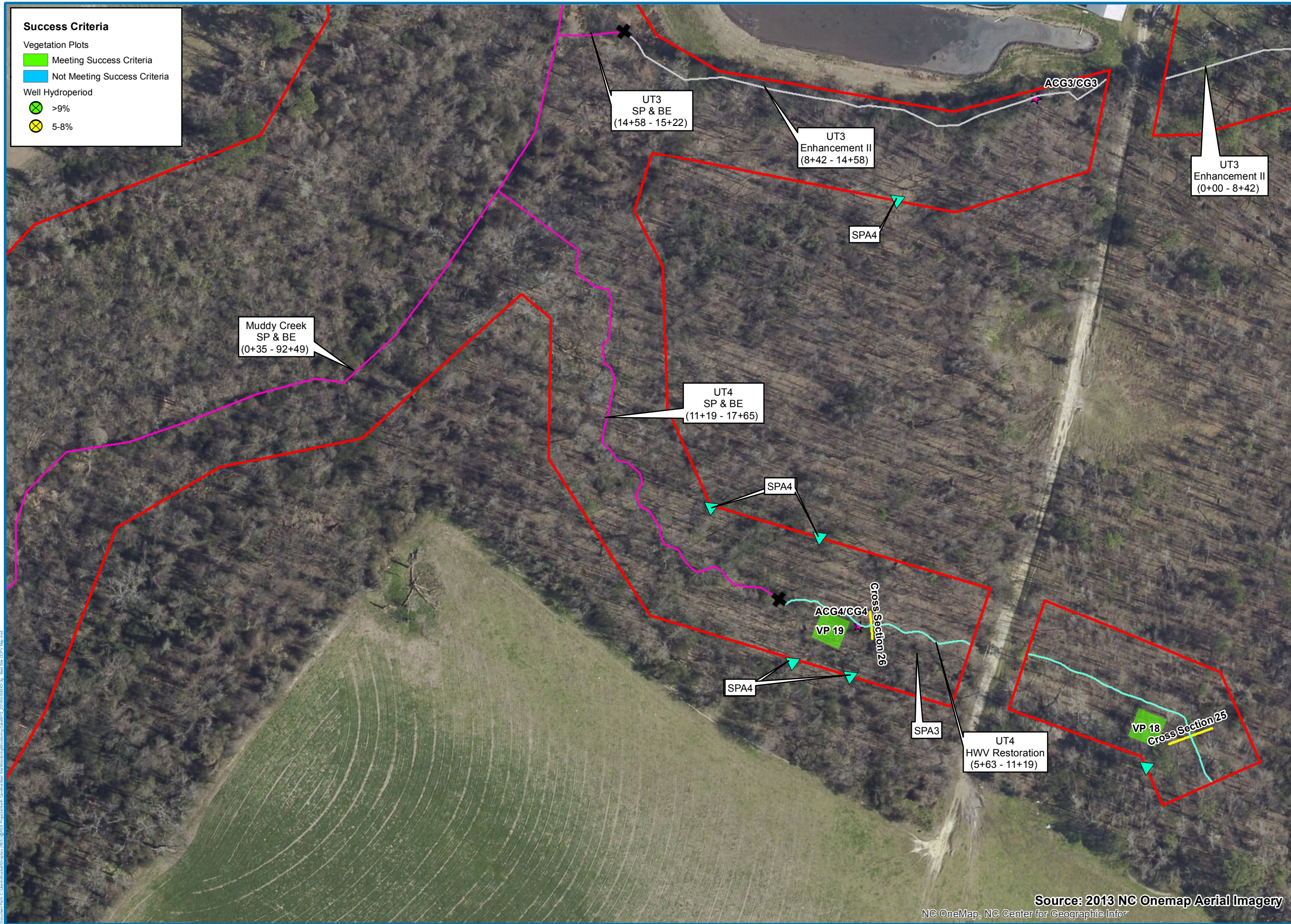
Figure 3g. Best Stream and Wetland Restoration Project UT4 & Muddy Creek Current Conditions Plan View Map
