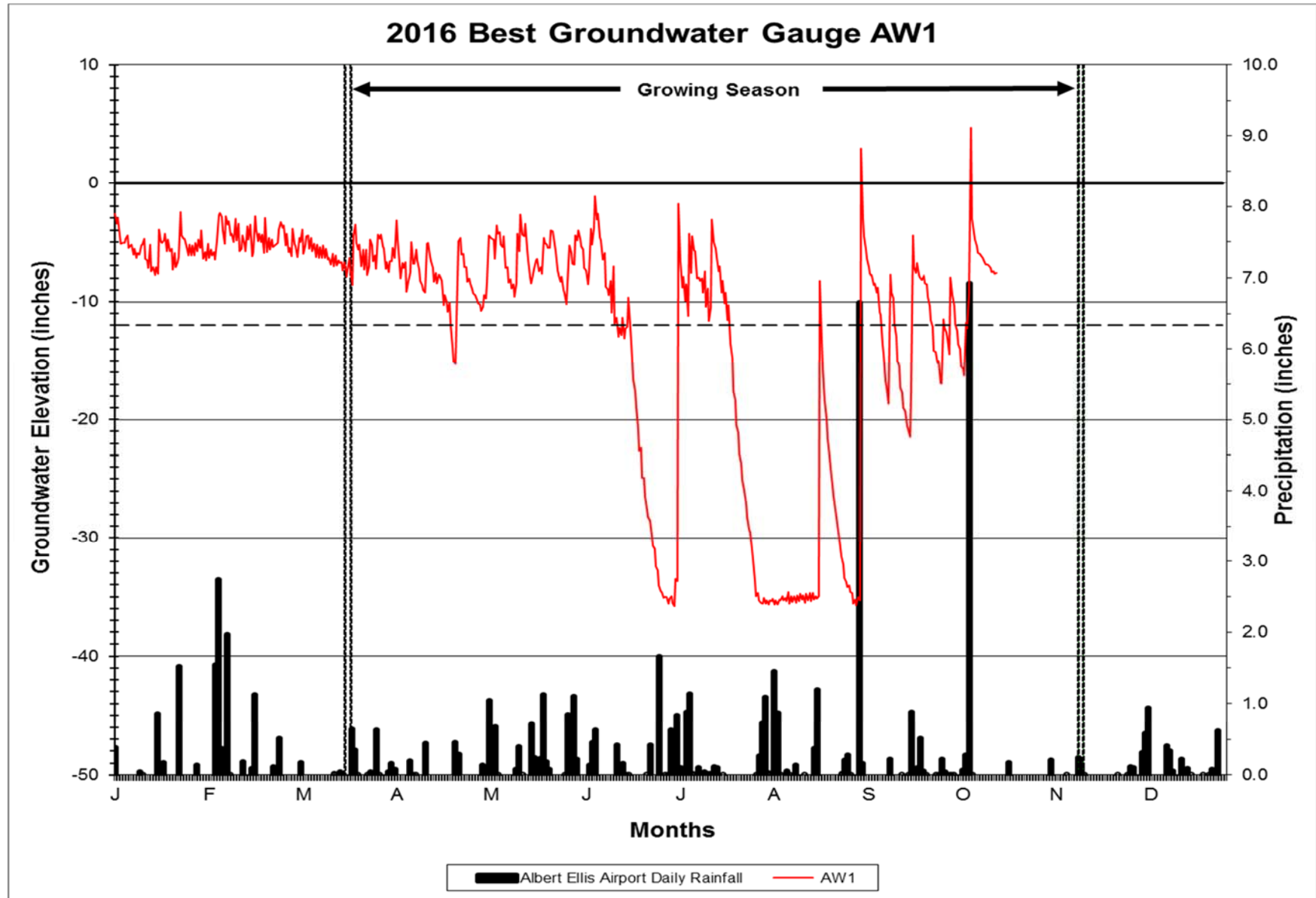
Chart 2. 2016 Best Site Groundwater Monitoring Gauge Hydrographs
