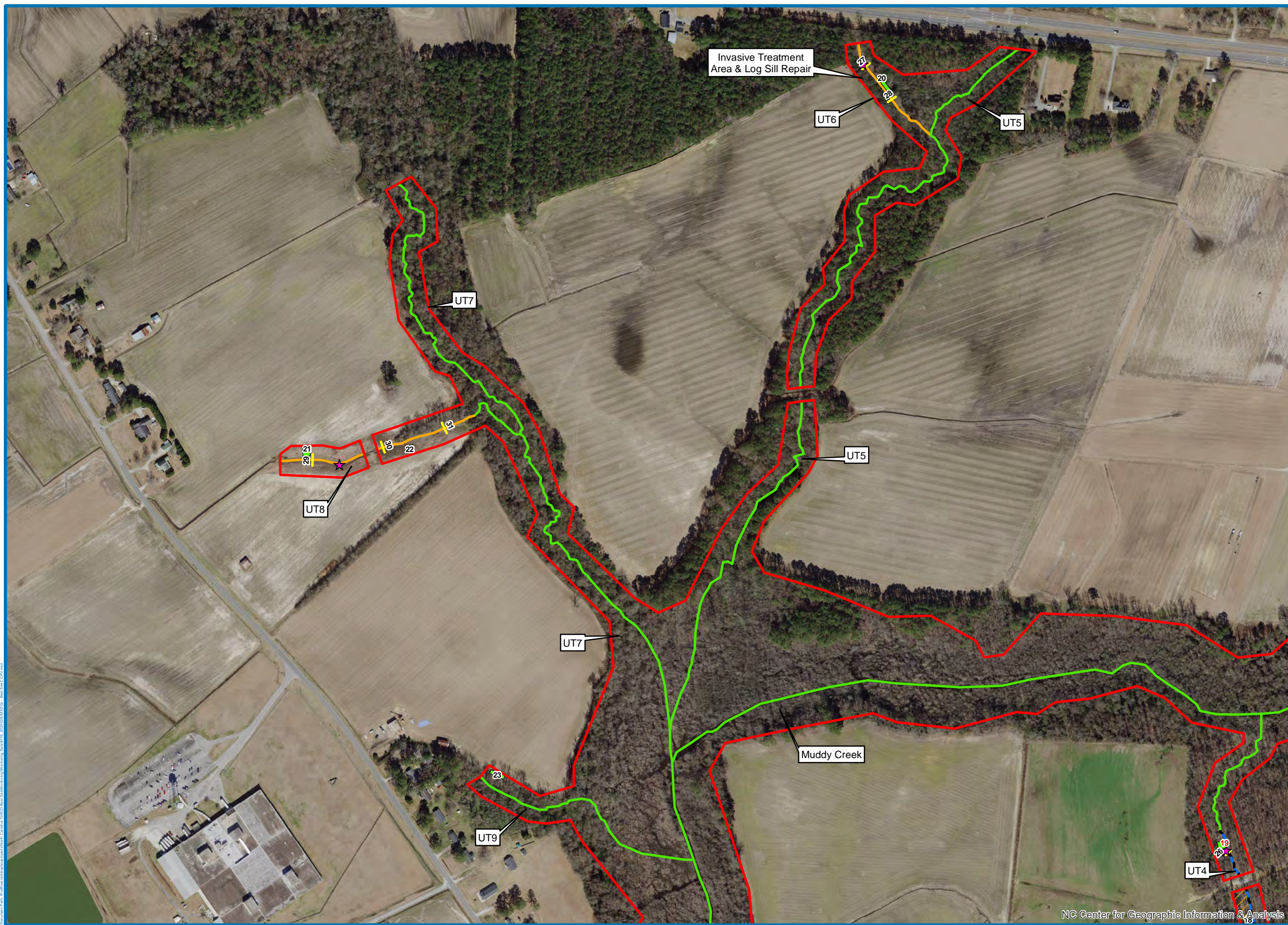
Figure 3c Best Stream and Wetland Restoration Project Current Conditions Plan View MY6 2020
