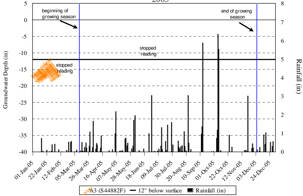
Figure 3. Hydrology Monitoring, Gauge A3 Dale Tract; Restoration 2005
