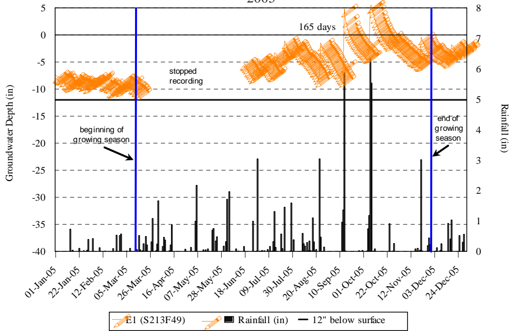
Figure 8. Hydrology Monitoring, Gauge E1 Dale Tract; Enhancement 2005
