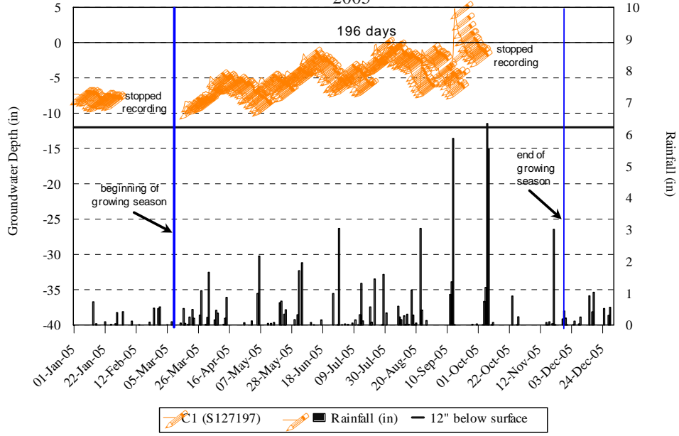
Figure 11. Hydrology Monitoring, Gauge C1 Dale Tract; Restoration 2005
