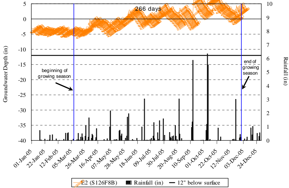
Figure 9. Hydrology Monitoring, Gauge E2 Dale Tract; Enhancement 2005
