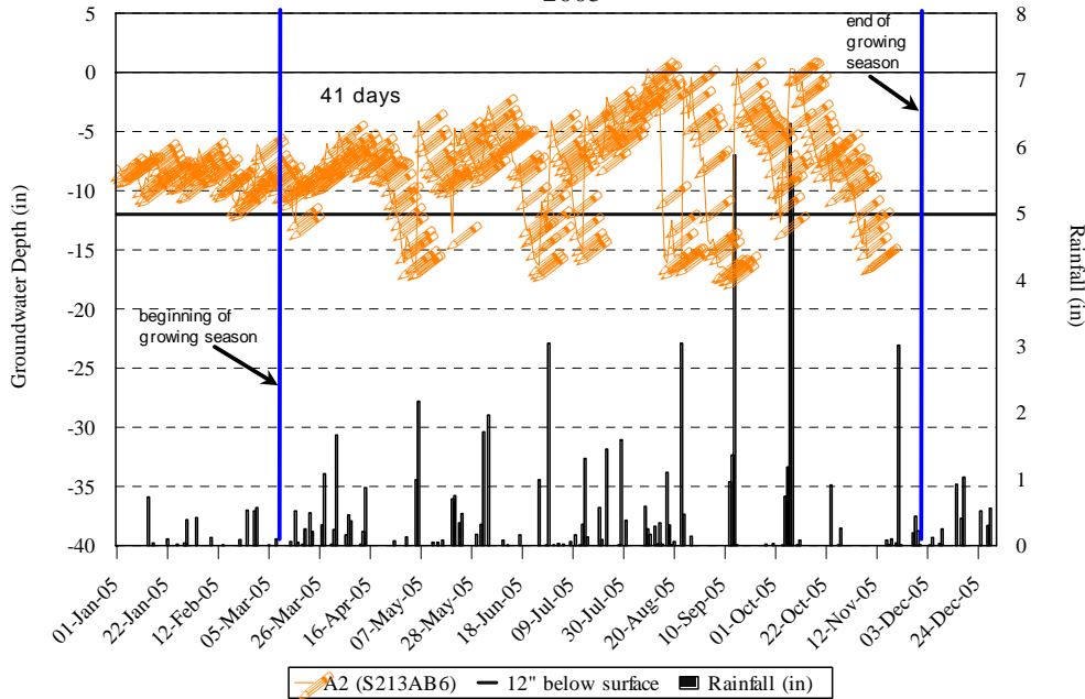
Figure 2. Hydrology Monitoring, Gauge A2 Dale Tract; Restoration 2005
