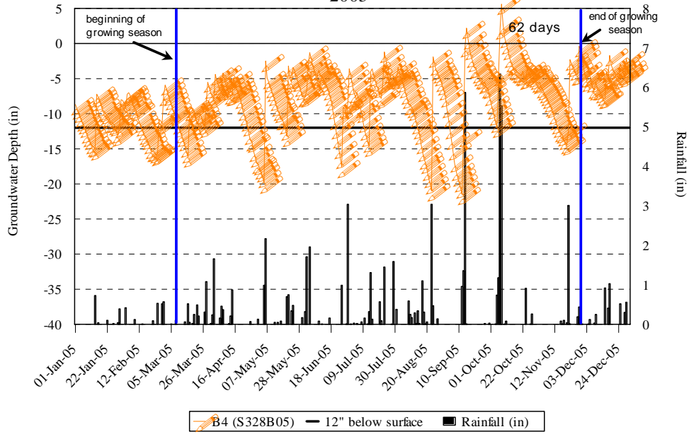
Figure 7. Hydrology Monitoring, Gauge B4 Dale Tract; Restoration 2005
