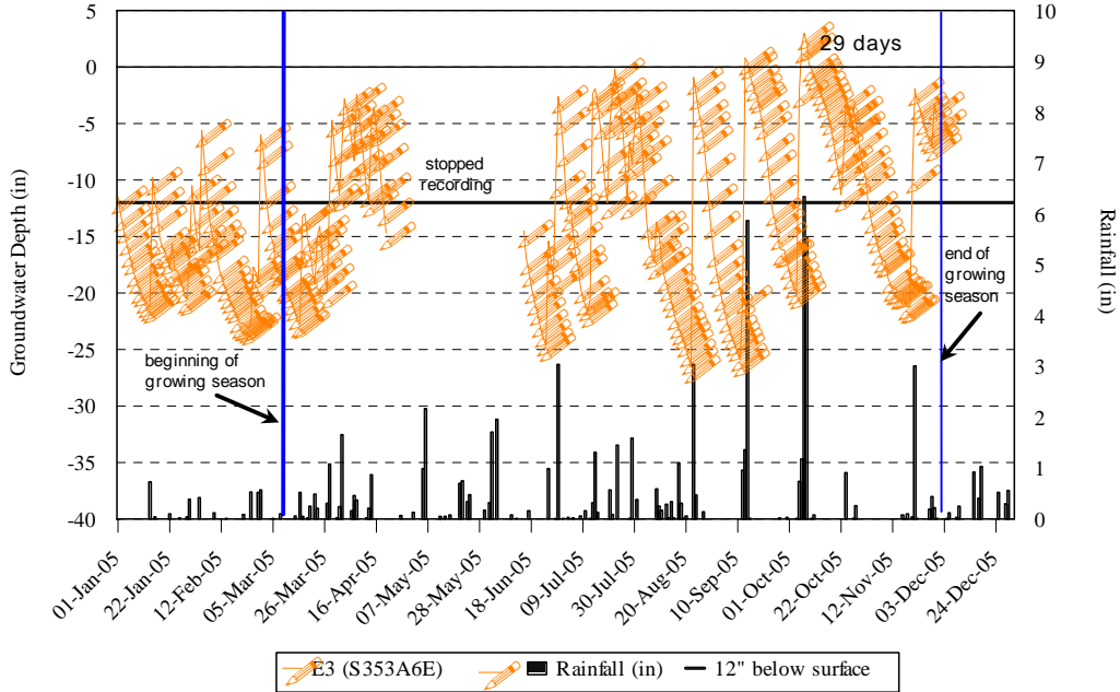
Figure 10. Hydrology Monitoring, Gauge E3 Dale Tract; Enhancement 2005
