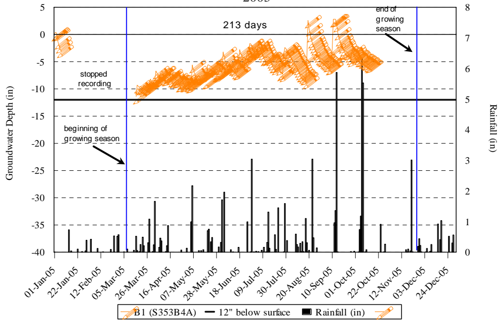
Figure 4. Hydrology Monitoring, Gauge B1 Dale Tract; Restoration 2005
