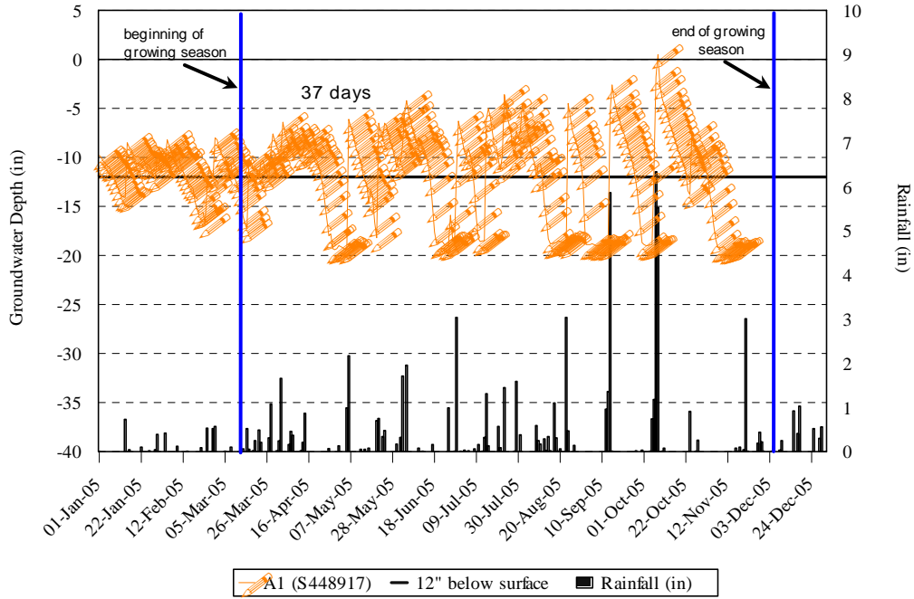
Figure 1. Hydrology Monitoring, Gauge A1 Dale Tract; Restoration 2005
