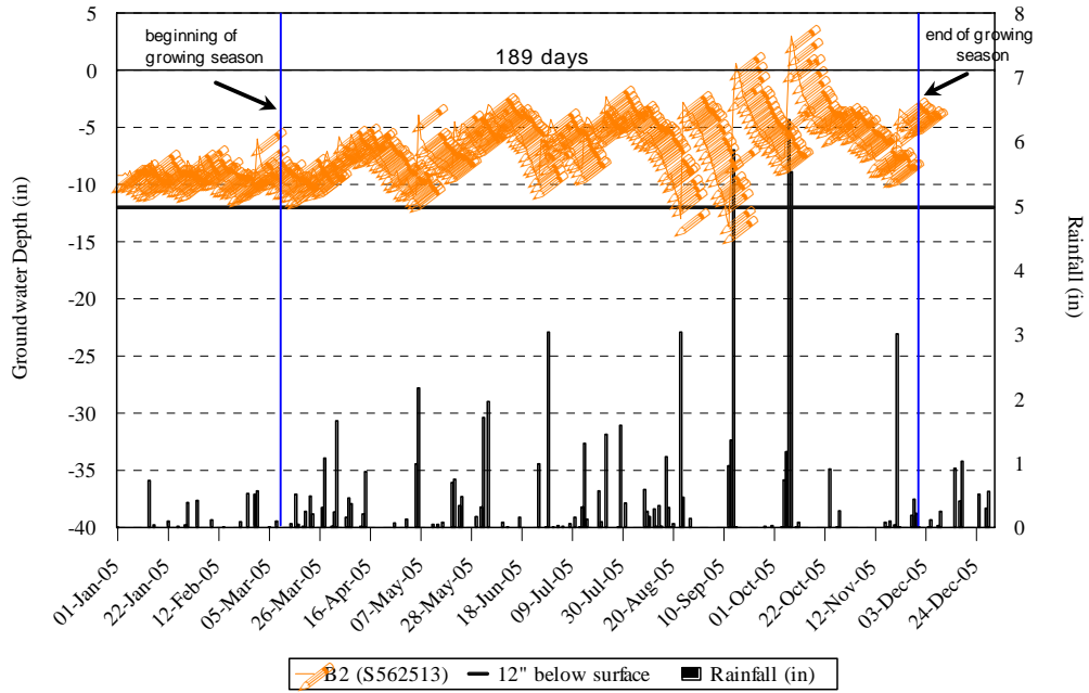
Figure 5. Hydrology Monitoring, Gauge B2 Dale Tract; Restoration 2005
