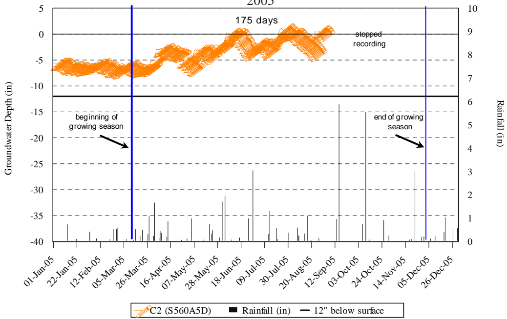
Figure 12. Hydrology Monitoring, Gauge C2 Dale Tract; Restoration 2005
