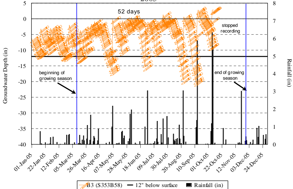
Figure 6. Hydrology Monitoring, Gauge B3 Dale Tract; Restoration 2005
