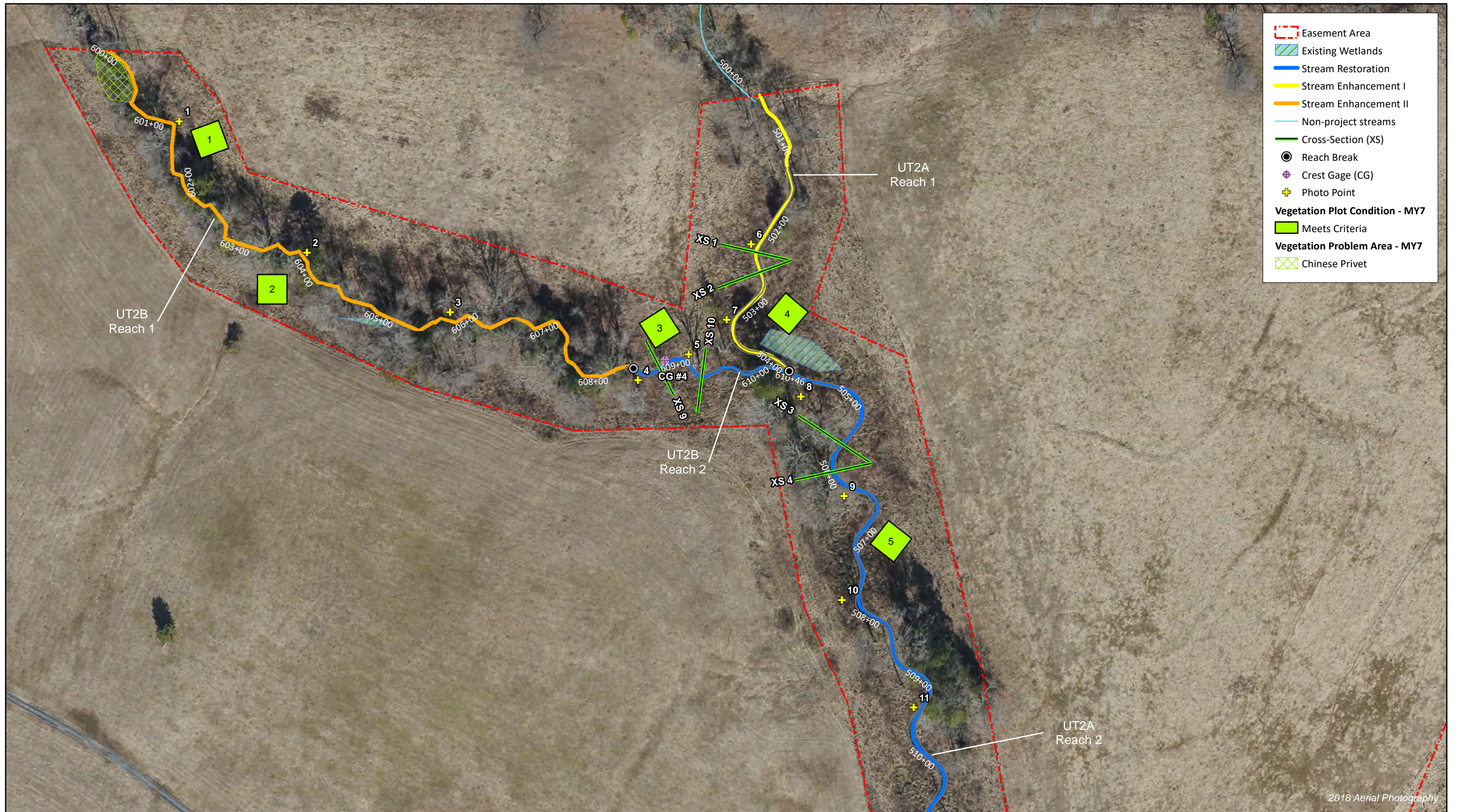
Figure 3.2 Integrated Current Condition Plan View (Sheet 2 of 7) Hopewell Stream Mitigation Site DMS Project No. 95352 Monitoring Year 7 - 2021 Randolph County
