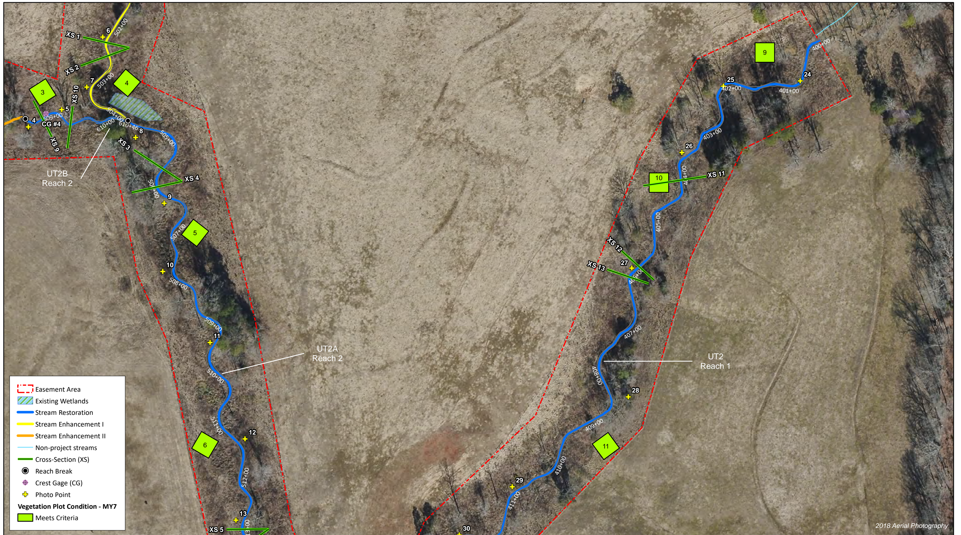
Figure 3.3 Integrated Current Condition Plan View (Sheet 3 of 7) Hopewell Stream Mitigation Site DMS Project No. 95352 Monitoring Year 7 - 2021 Randolph County
