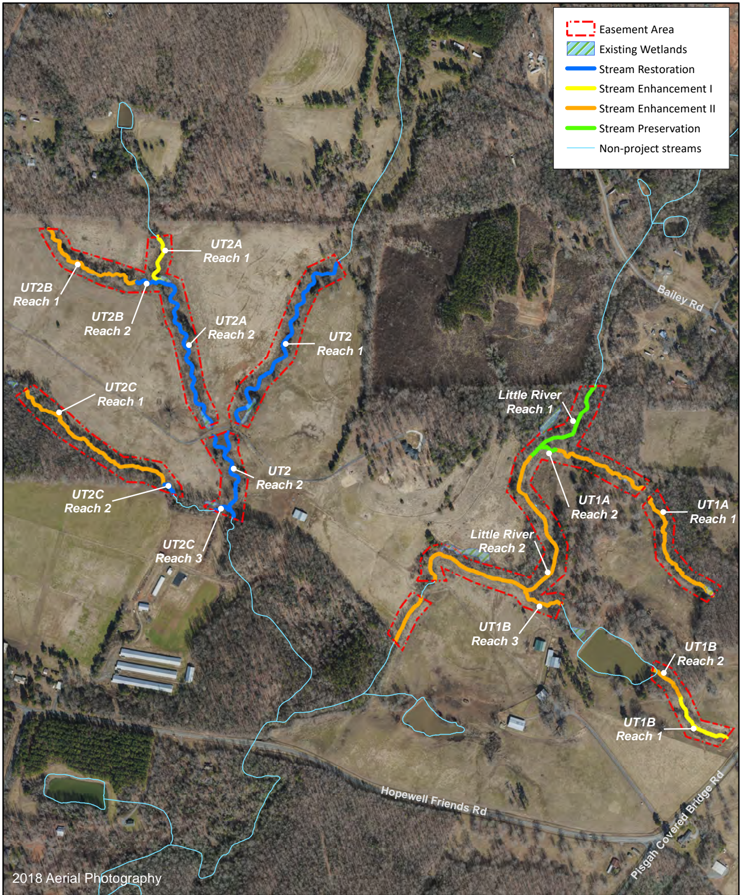
Figure 2 Project Component Map Hopewell Stream Mitigation Site DMS Project No. 95352 Monitoring Year 7 - 2021 Randolph County, NC
