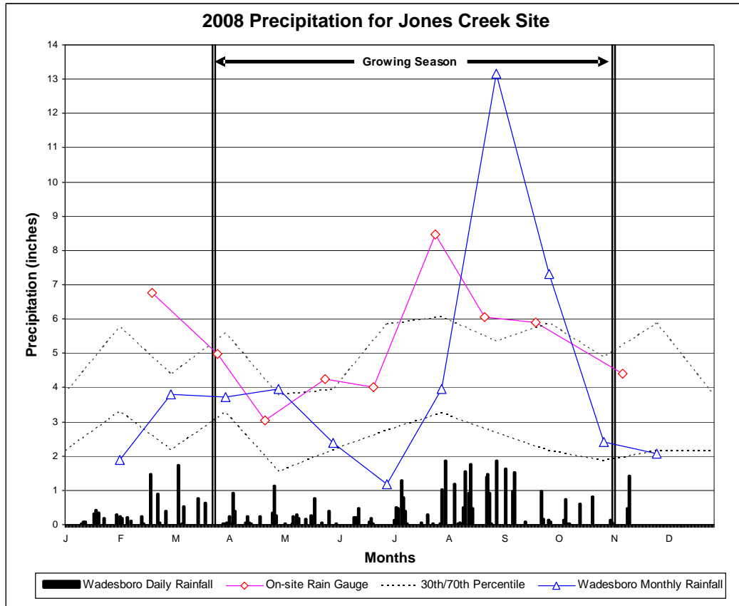
Figure 6. 2008 Rainfall
