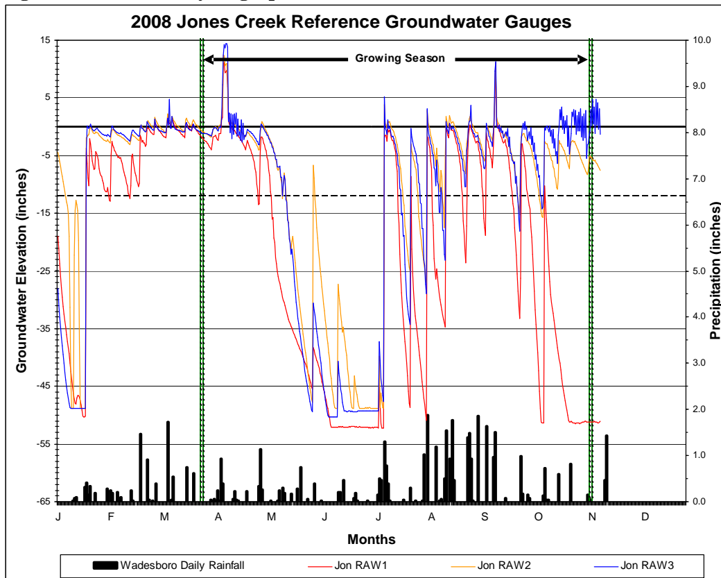
Figure 5. Reference Hydrographs
