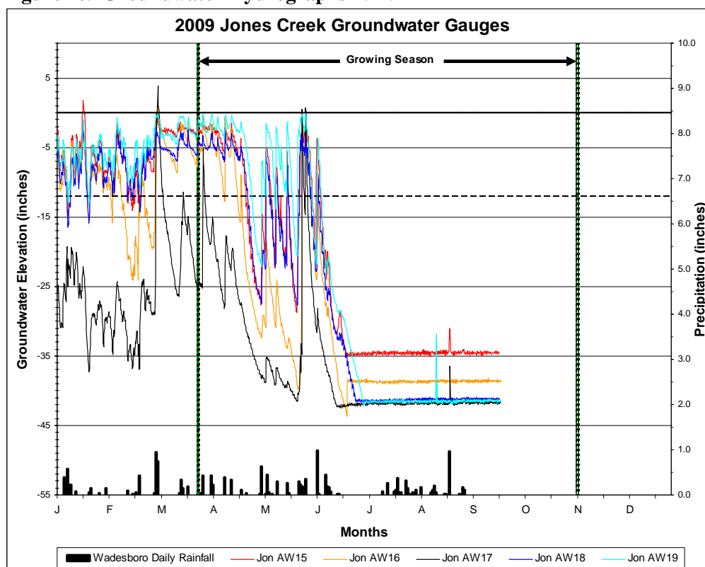
Figure 4e. Groundwater Hydrographs 15-19
