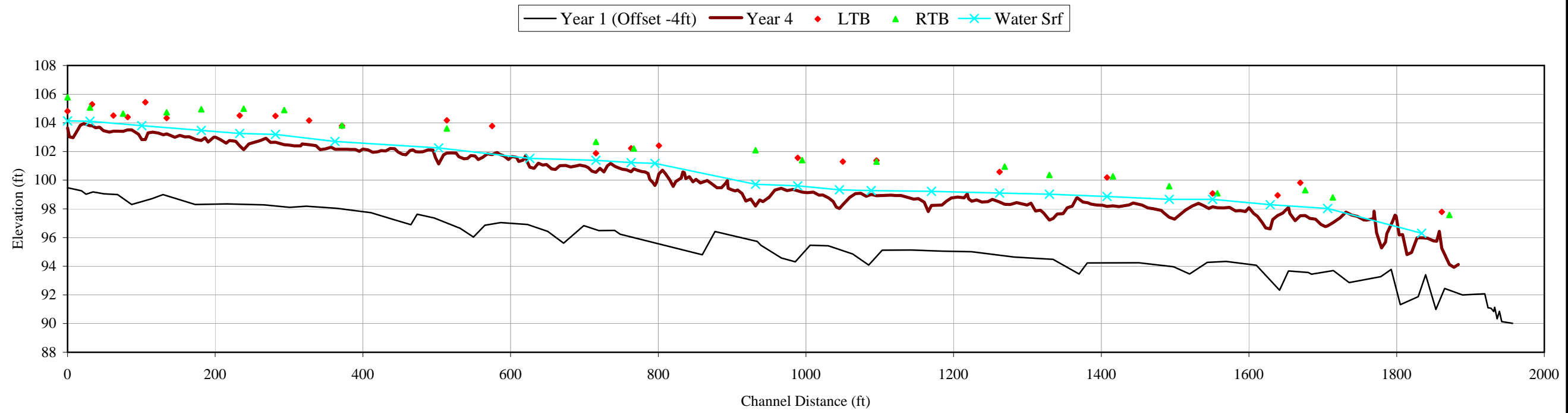
Jones Creek UT 2009 Profile
