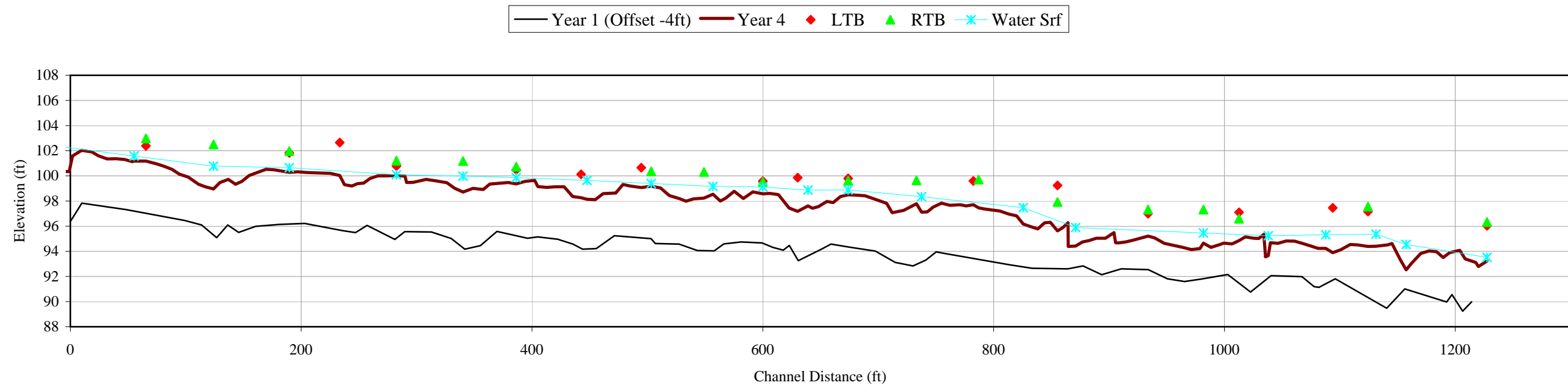
Jones Creek UT 2009 Profile
