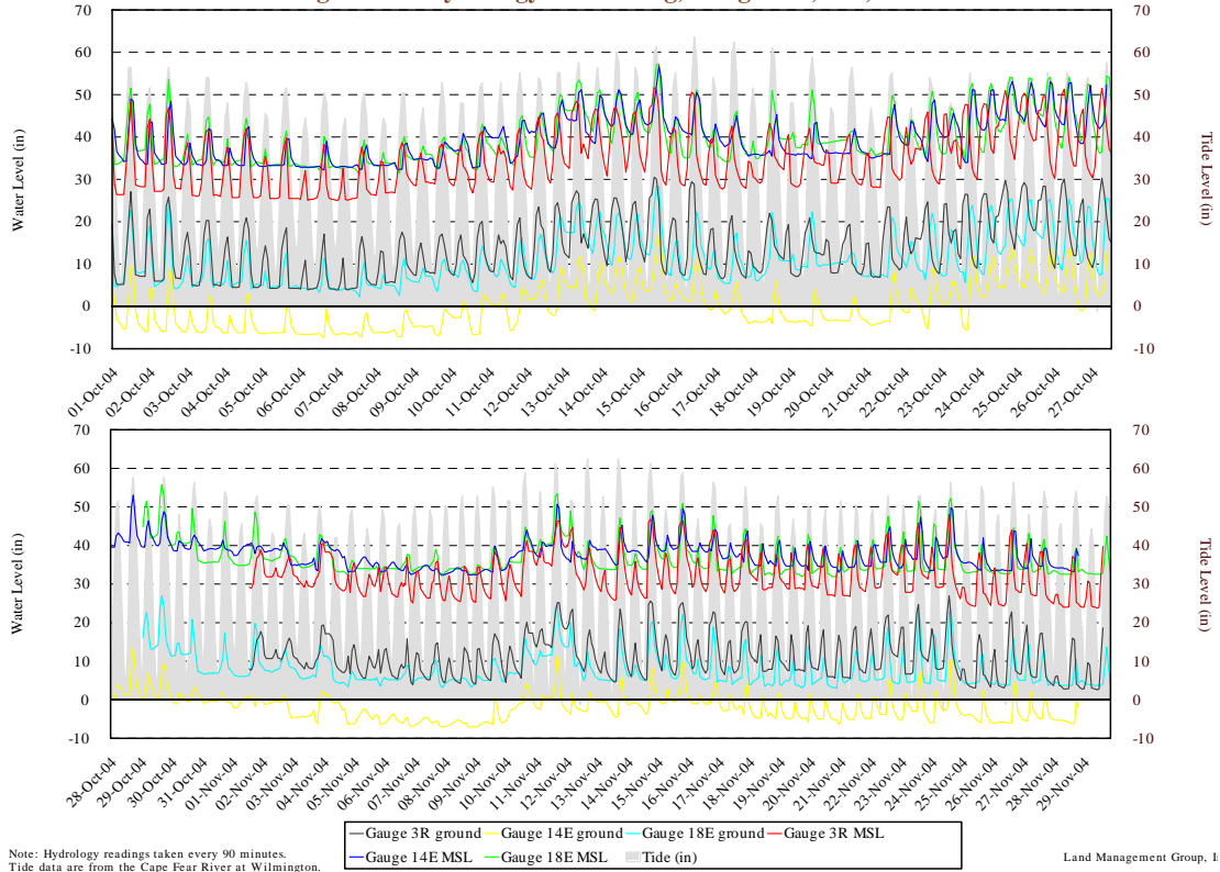
Figure B.3. Hydrology Monitoring, Gauges 3R, 14E, and 18E
