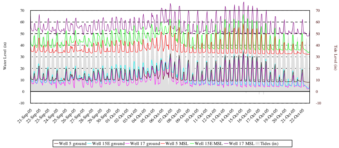
Figure B.6 contd. Hydrology Monitoring, Gauges 5R, 15E, and 17
