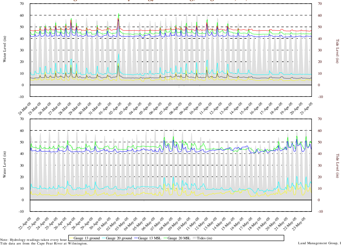
Figure B.8 contd. Hydrology Monitoring, Gauges 21R, 13, and 20
