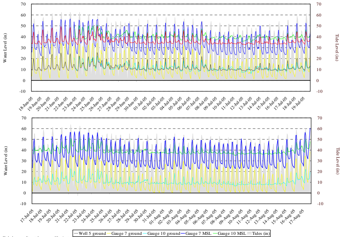
Figure B.5 contd. Hydrology Monitoring, Gauges 5R, 7, and 10
