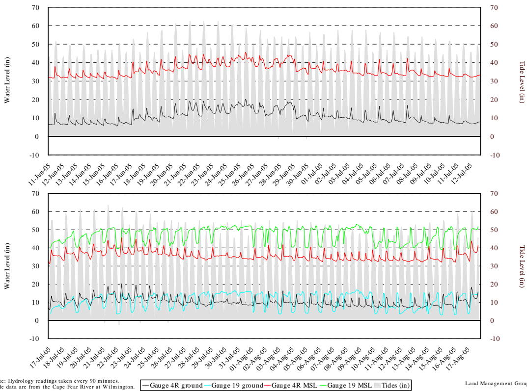
Figure B.4 contd. Hydrology Monitoring, Gauges 4R and 19
