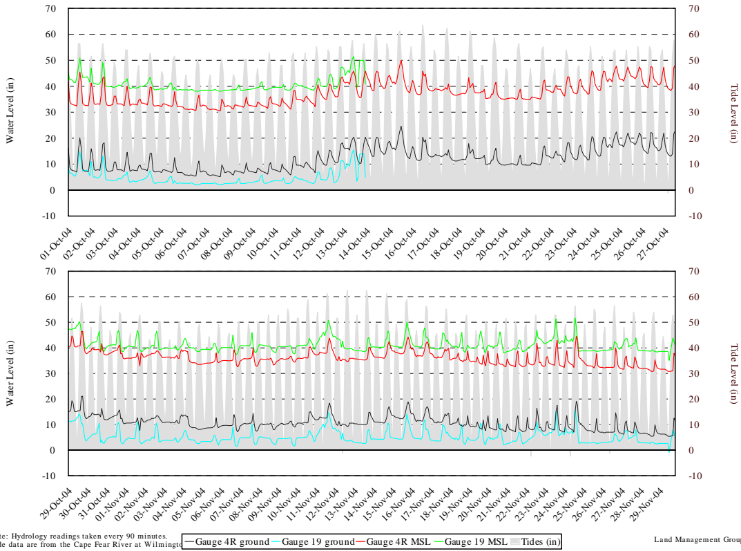
Figure B.4. Hydrology Monitoring, Gauges 4R and 19
