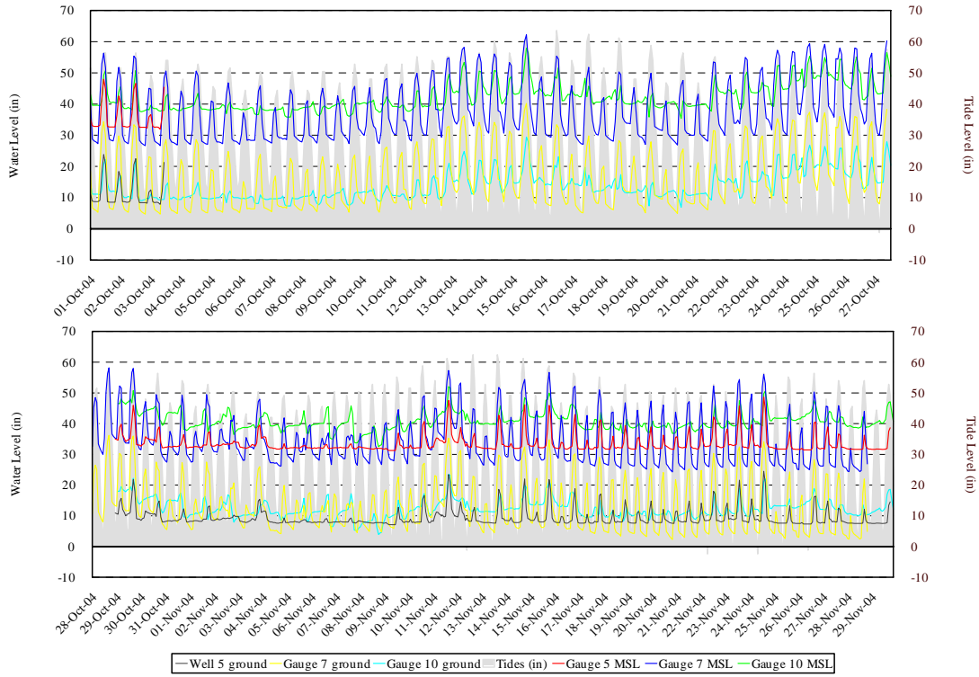
Figure B.5. Hydrology Monitoring, Gauges 5R, 7, and 10
