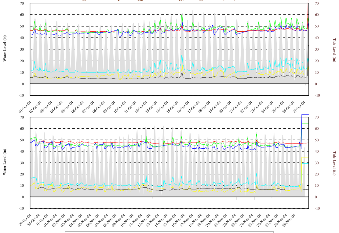
Figure B.8. Hydrology Monitoring, Gauges 21R, 13, and 20
