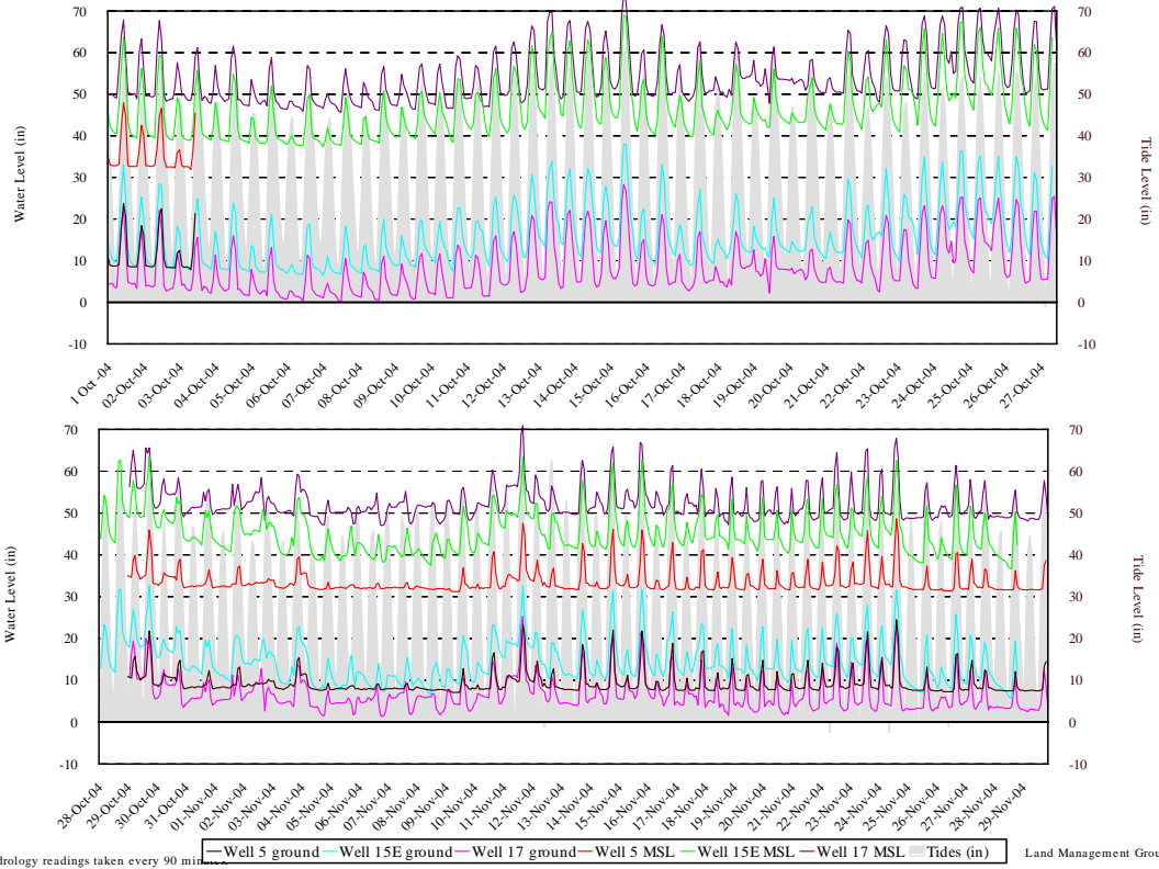
Figure B.6. Hydrology Monitoring, Gauges 5R, 15E, and 17
