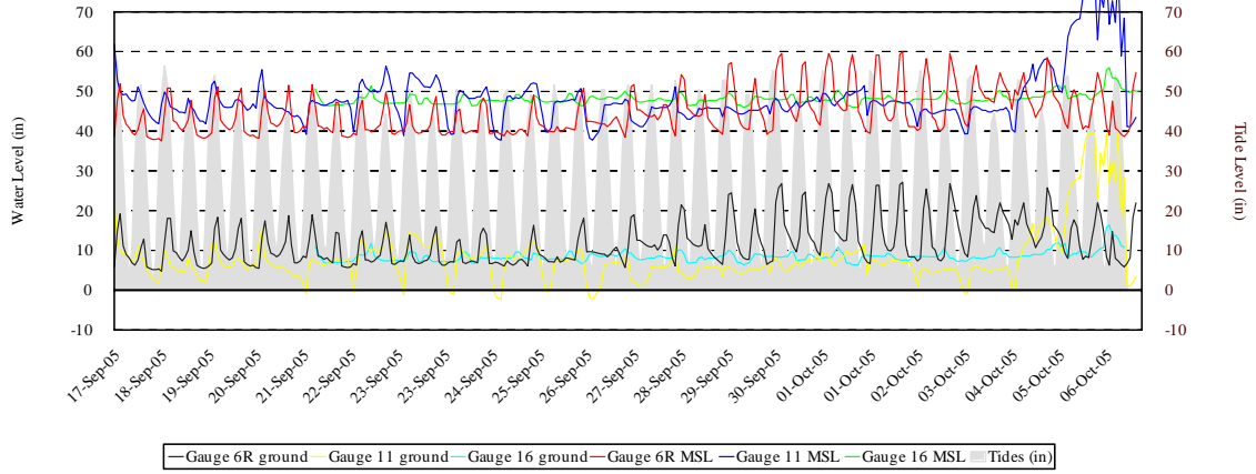
Figure B.7 contd. Hydrology Monitoring, Gauges 6R, 11, and 16
