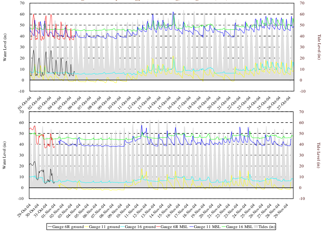
Figure B.7. Hydrology Monitoring, Gauges 6R, 11, and 16
