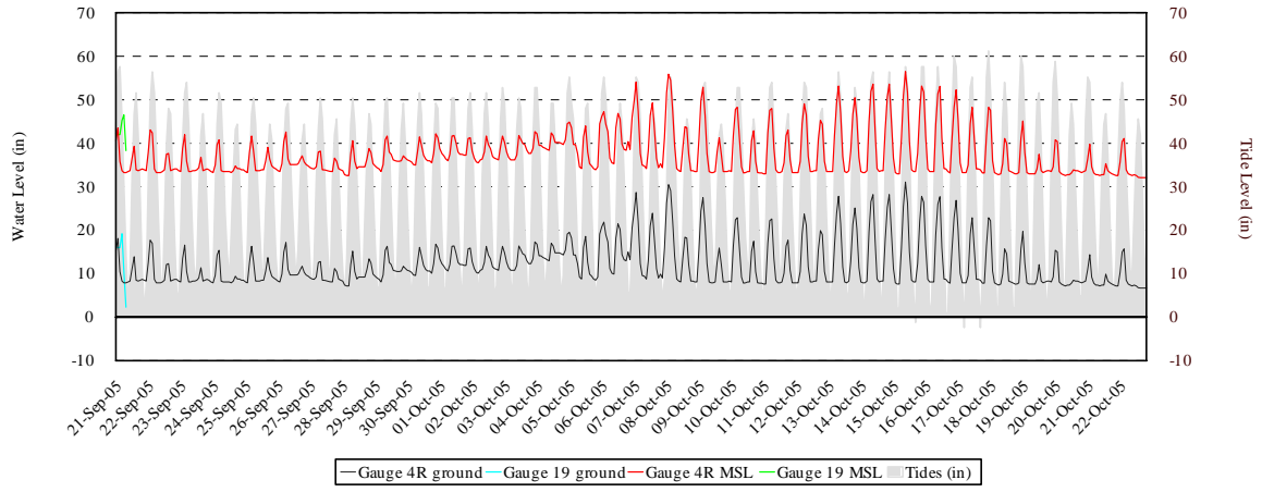
Figure B.4 contd. Hydrology Monitoring, Gauges 4R and 19
