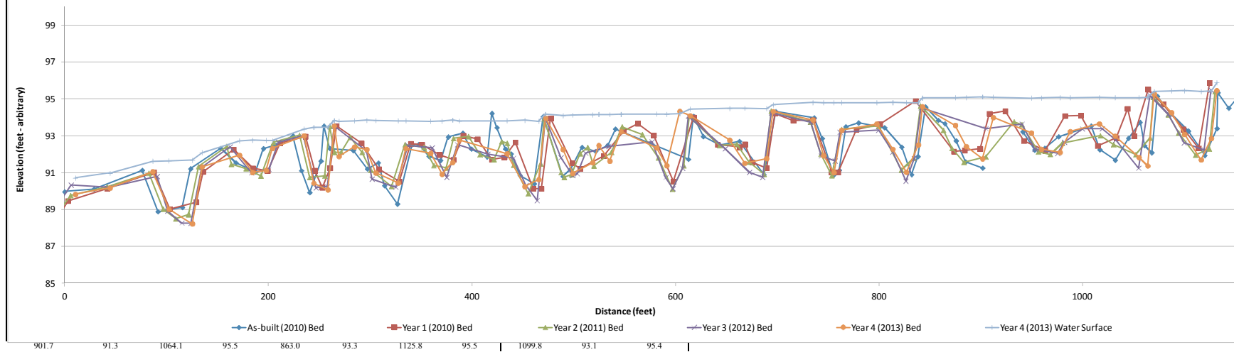
McIntyre Creek Year 4 (2013) Profile - Reach 00+00 to 11+50
