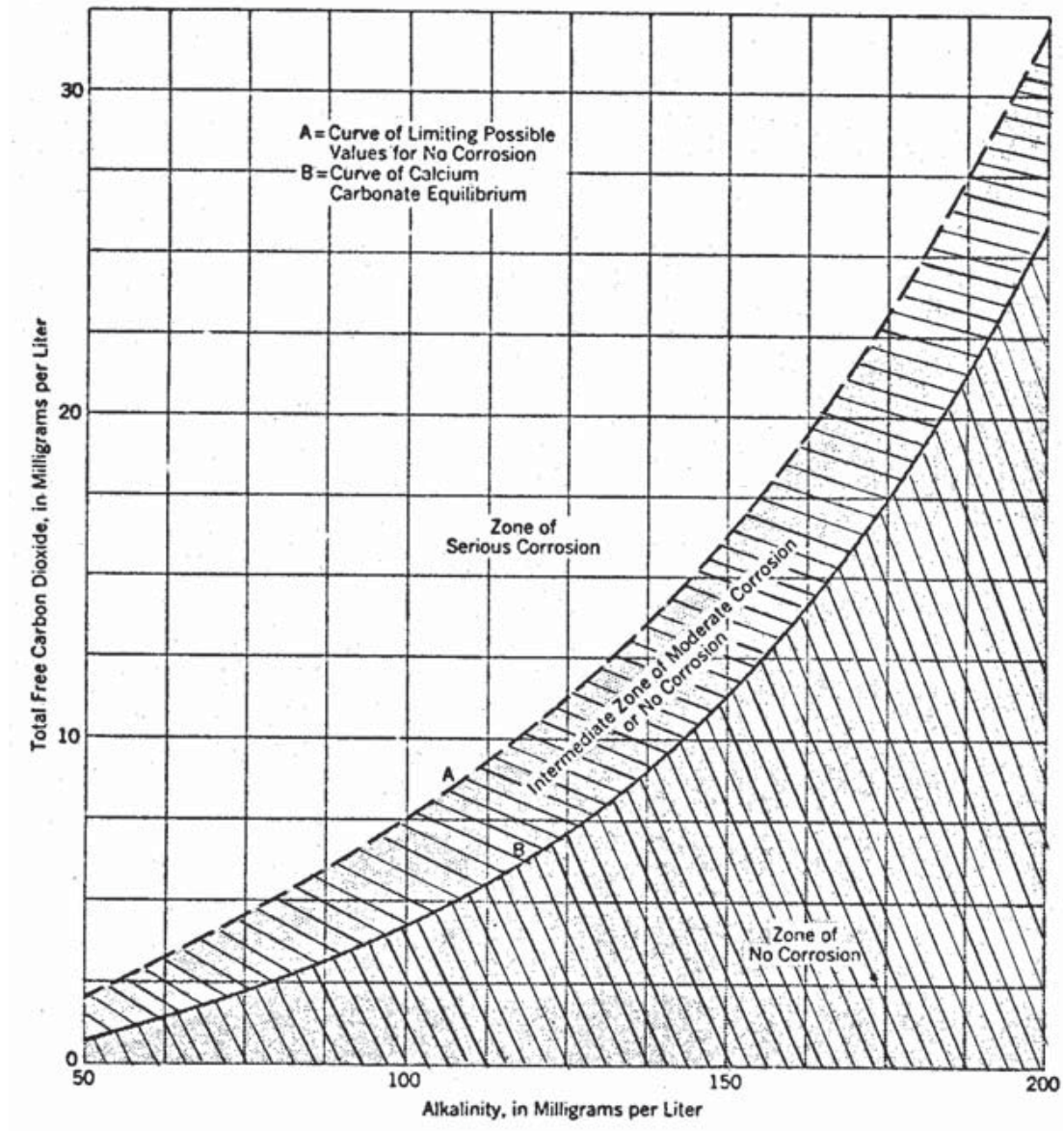
FIGURE 1(B) ALKALINITY VS TOTAL FREE CARBON DIOXIDE
