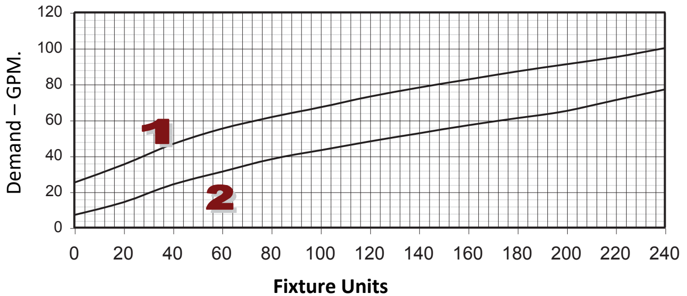
FIGURE 3(D): ENLARGED SCALE DEMAND LOAD
