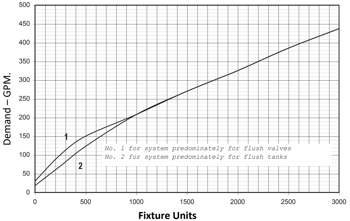
FIGURE 3(D): ENLARGED SCALE DEMAND LOAD
