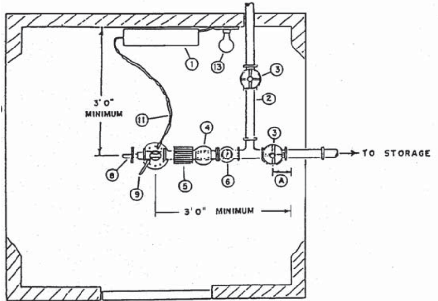
FIGURE 4: TYPICAL WELL HEAD DETAILS
