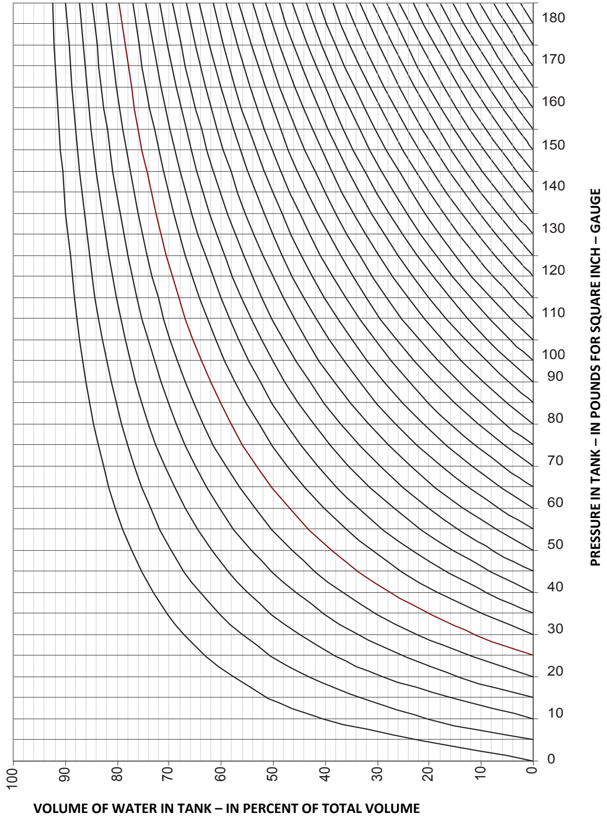
FIGURE 5: PRESSURE & VOLUME DIFFERENTIALS FOR HYDROPNEUMATIC TANKS
