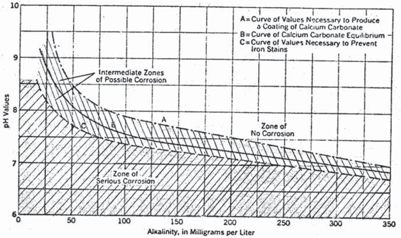
FIGURE 1(A) ALKALINITY VS pH
