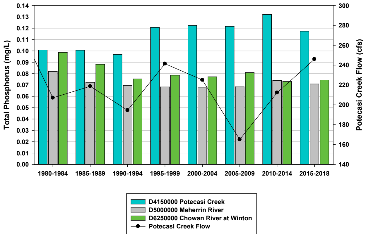
Figure 5-36: Five-Year Mean TP Concentrations and Flow at the Potecasi Creek (D4150000), Meherrin River (D5000000) and Chowan River at Winton (D6250000) AMS Stations. (Potecasi Creek Flow at USGS Gage 02053200; Co-located with AMS Station D4150000.)
