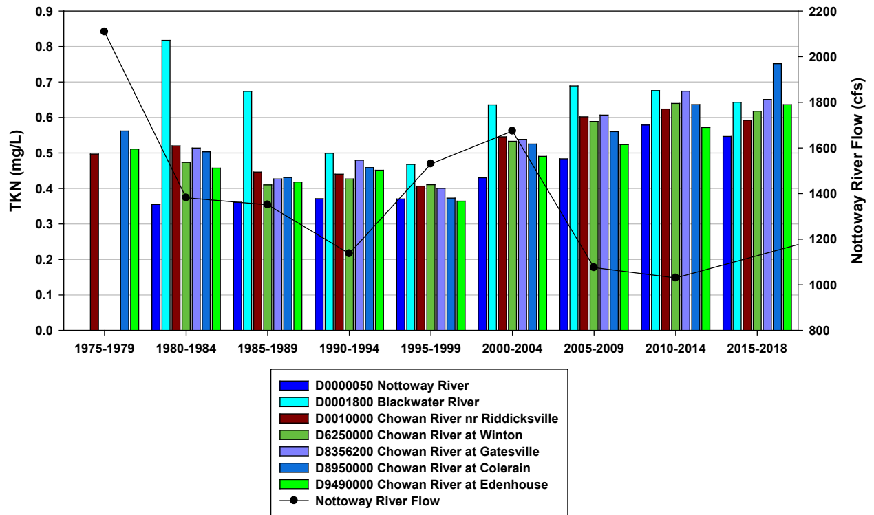
Figure 5-25: Five Year Mean TKN Concentrations and Nottoway River Flow (1975-2018).
