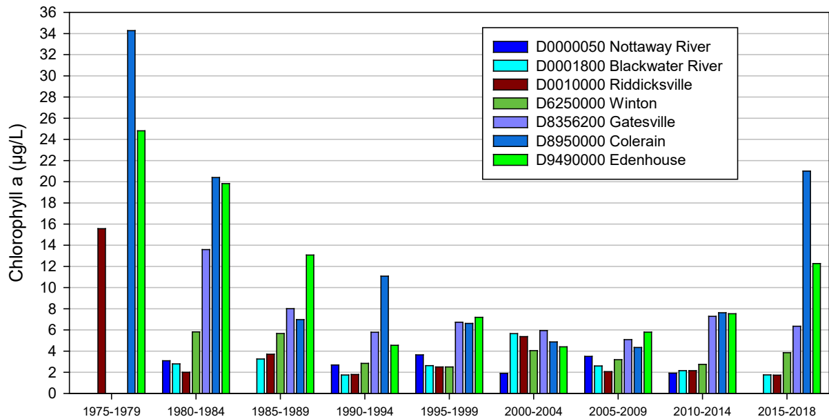
Figure 5-39: Chowan River Five Year Mean Chlorophyll a Concentrations at Two VA and Five NC Mainstem Chowan River Stations. (No Chlorophyll a Data Available Between September 1996 - March 2001.)
