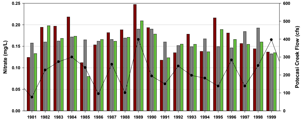
Figure 5-14: Annual Mean Nitrate Concentrations Comparison Between the Meherrin River Station and the Chowan River Upstream and Downstream Confluence Stations for (a) Years 1981-1999 and (b) Years 2000-2018.
