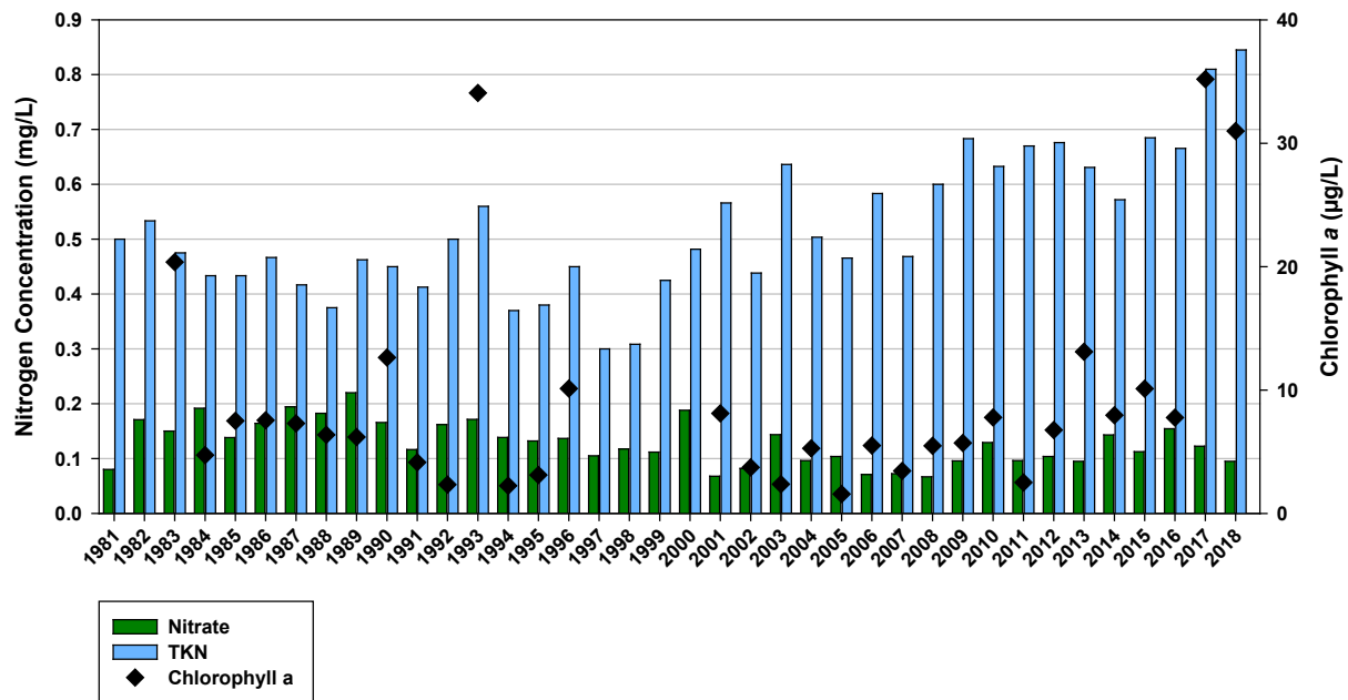
Figure 5-29: Annual Mean TKN, Nitrate and Chlorophyll a Concentrations at D8950000, Chowan River at Colerain.
