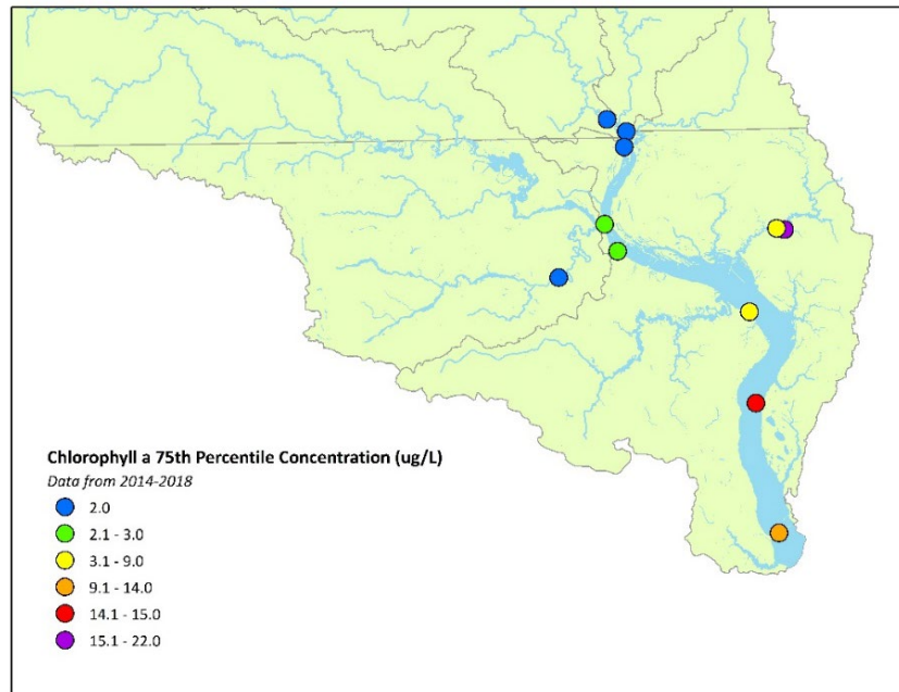
Figure 5-37: Chowan River Basin AMS and Lake Stations 2020 IR Period (2014-2018) Chlorophyll a (a) 75th Percentile Concentrations and (b) Percent Exceedances of the Standard (40 µg/L).
