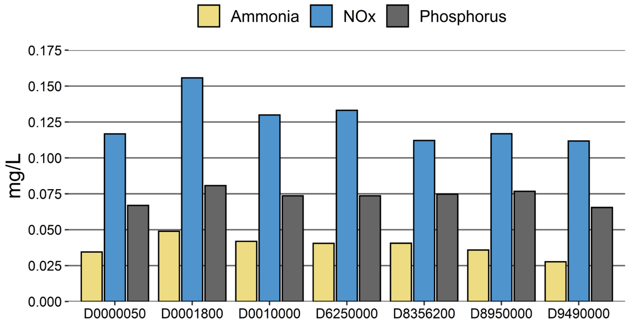
Figure 5-5: The 2010 - 2018 Mean Nutrient Concentrations for Mainstem Stations Including the Virginia Stations (D0000050 & D0001800). (a) Means for Ammonia, Nitrate (NOx) and Phosphorus (b) Means for Ammonia, Nitrate (NOx), Phosphorus and Total Kjeldahl Nitrogen (TKN).
