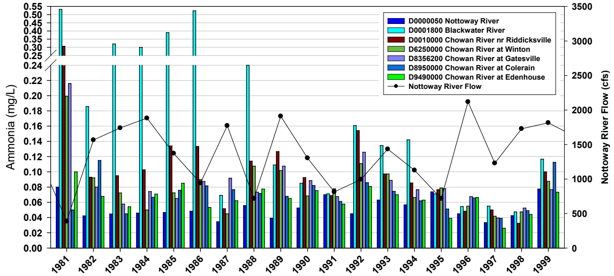
Figure 5-19: Annual Mean Ammonia Concentrations with Annual Nottoway River Flow ((a) 1981-1999 and (b) 2000-2018) (Note the ammonia axis scale break, this is the same axis for both a and b) (c) 2006-2018 (This time frame focuses on the most recent instream ammonia concentration, note both Y-axis change to allow for better visual evaluation of the change that has occurred over this time period).
