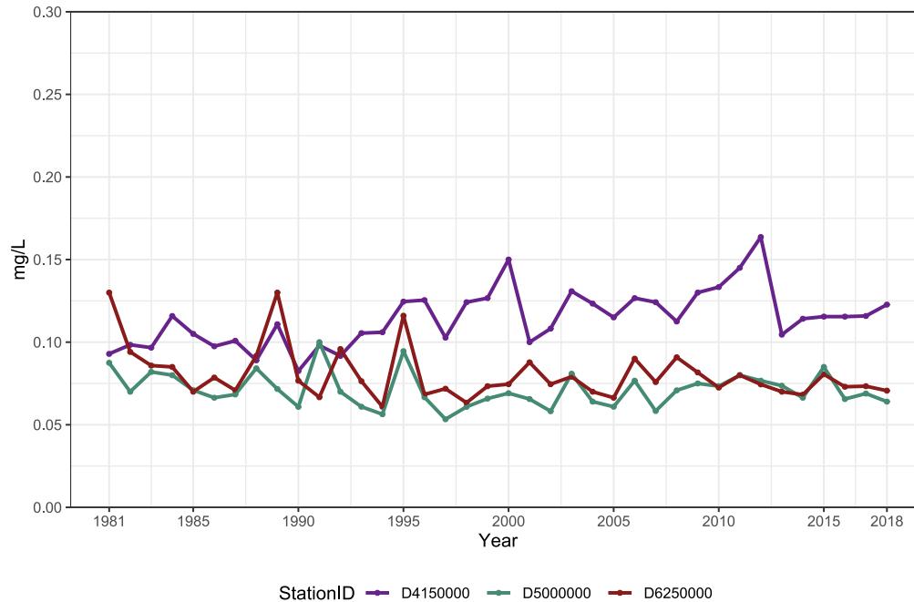
Phosphorus - Chowan River Annual Mean Values 1981 - 2018
