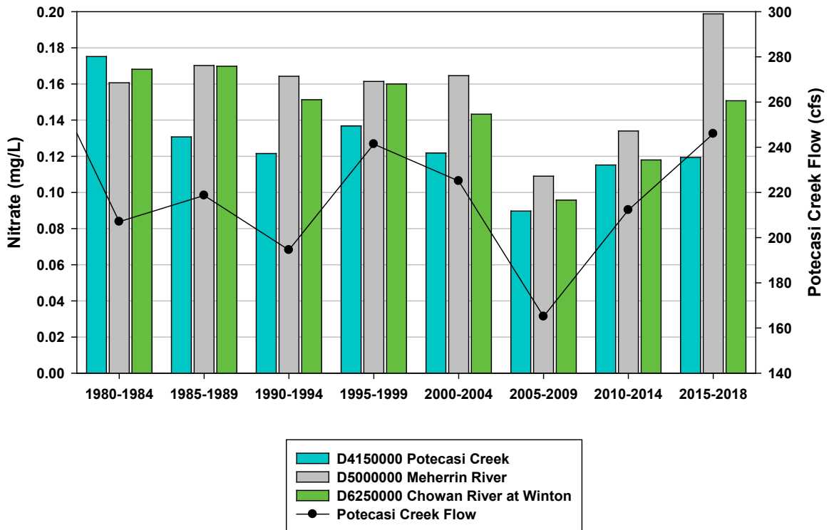
Figure 5-16: Five-Year Mean Nitrate Concentrations and Flow at the Potecasi Creek (D4150000), Meherrin River (D5000000) and Chowan River at Winton (D6250000) AMS Stations. (Flow at USGS Gage 02053200; Co-located with AMS Station D4150000.)
