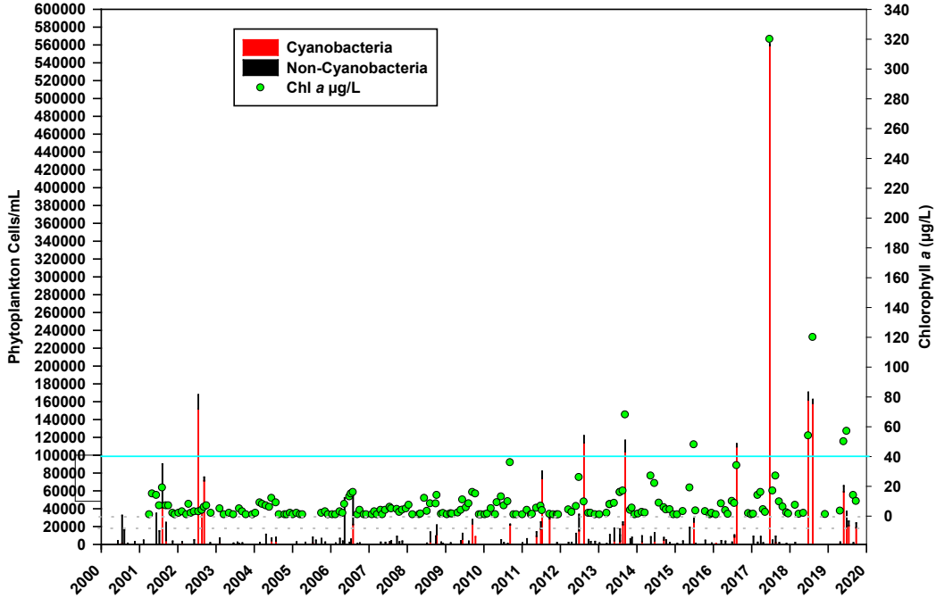
Figure 5-41: Chowan River at Colerain (D8950000) Chlorophyll a Concentration and Phytoplankton Counts (Cyanobacteria and Non-Cyanobacteria Cell Densities). (a) 2000-2019 (No Axis Break), (b) 2000-2019 with Y-Axis Breaks, (c) 2010-2019 with Y-Axis Breaks.
