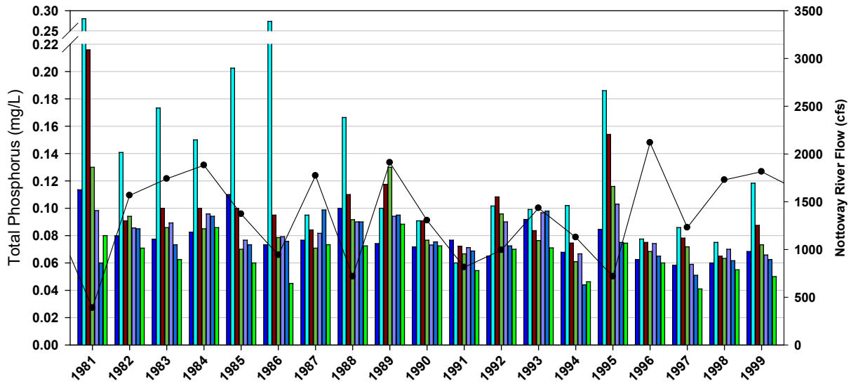
Figure 5-31: Annual Mean TP Concentrations with Annual Nottoway River Flow (a) 1981-1999, (b) 2000-2018 with the 2008 Year Inset to Display a High Spike in the Blackwater River and the Corresponding Watershed Response. (Note the TP axis scale break, this is the same axis for both graphs).
