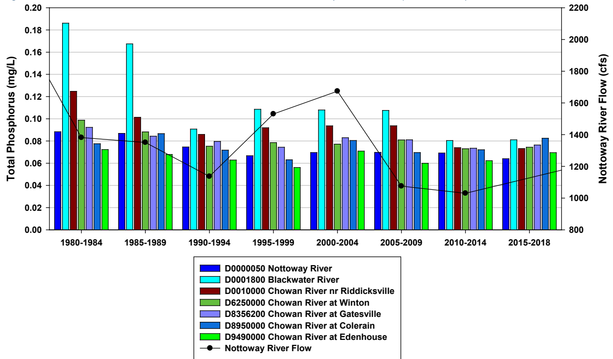
Figure 5-33: Five Year Mean TP Concentrations and Nottoway River Flow (1980-2018).
