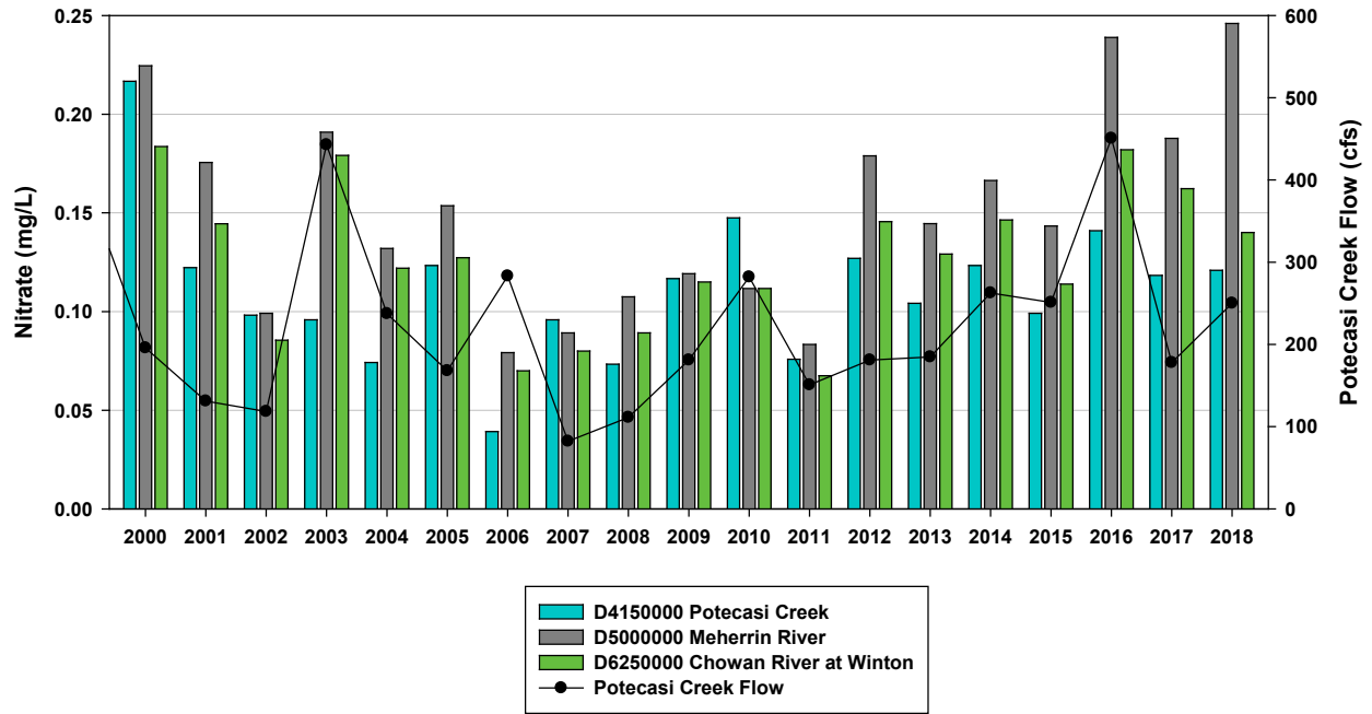
Figure 5-16: Five-Year Mean Nitrate Concentrations and Flow at the Potecasi Creek (D4150000), Meherrin River (D5000000) and Chowan River at Winton (D6250000) AMS Stations. (Flow at USGS Gage 02053200; Co-located with AMS Station D4150000.)
