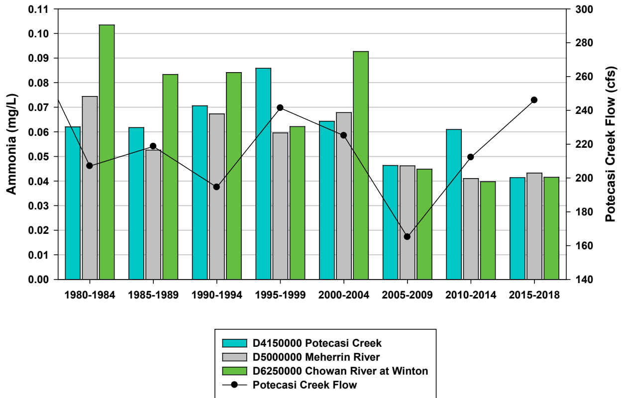
Figure 5-22: Five-Year Mean Ammonia Concentrations and Flow at the Potecasi Creek (D4150000), Meherrin River (D5000000) and Chowan River at Winton (D6250000) AMS Stations. (Flow at USGS Gage 02053200; Co-located with AMS Station D4150000).
