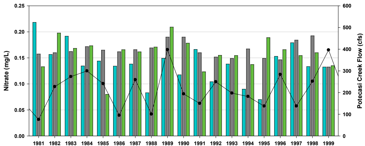
Figure 5-15: Annual Mean Nitrate Concentrations and Flow at the Potecasi Creek (D4150000), Meherrin River (D5000000) and Chowan River at Winton (D6250000) AMS Stations for Comparison for (a) Years 1981-1999 and (b) Years 2000-2018. (Flow at USGS Gage 02053200; Co-located with AMS Station D4150000.)
