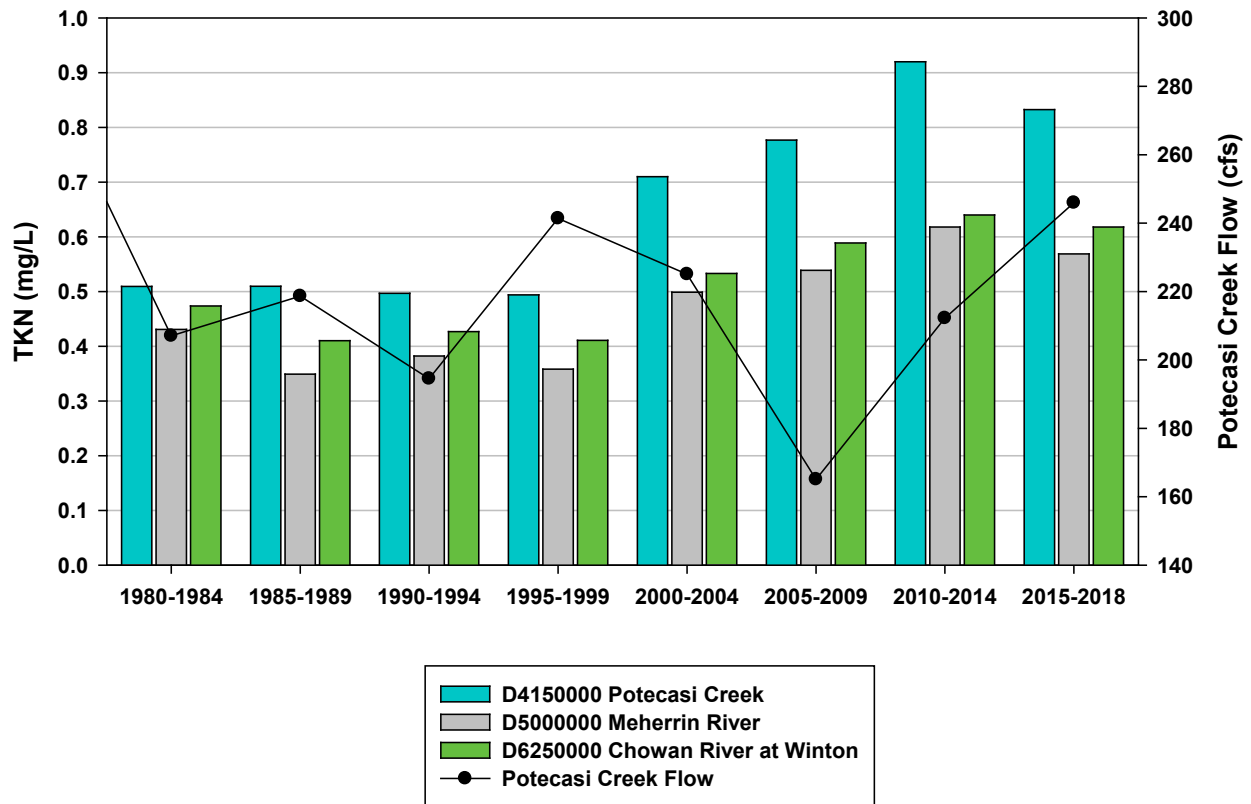
Figure 5-28: Five-Year Mean TKN Concentrations and Flow at the Potecasi Creek (D4150000), Meherrin River (D5000000) and Chowan River at Winton (D6250000) AMS Stations. (Potecasi Creek Flow at USGS Gage 02053200; Co-located with AMS Station D4150000).
