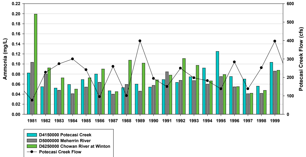
Figure 5-21: Annual Mean Ammonia Concentration and Flow at the Potecasi Creek (D4150000), Meherrin River (D5000000) and Chowan River at Winton (D6250000) AMS Stations for Comparison for (a) Years 1981-1999 and (b) Years 2000-2018. (Flow at USGS Gage 02053200; Co-located with AMS Station D4150000).
