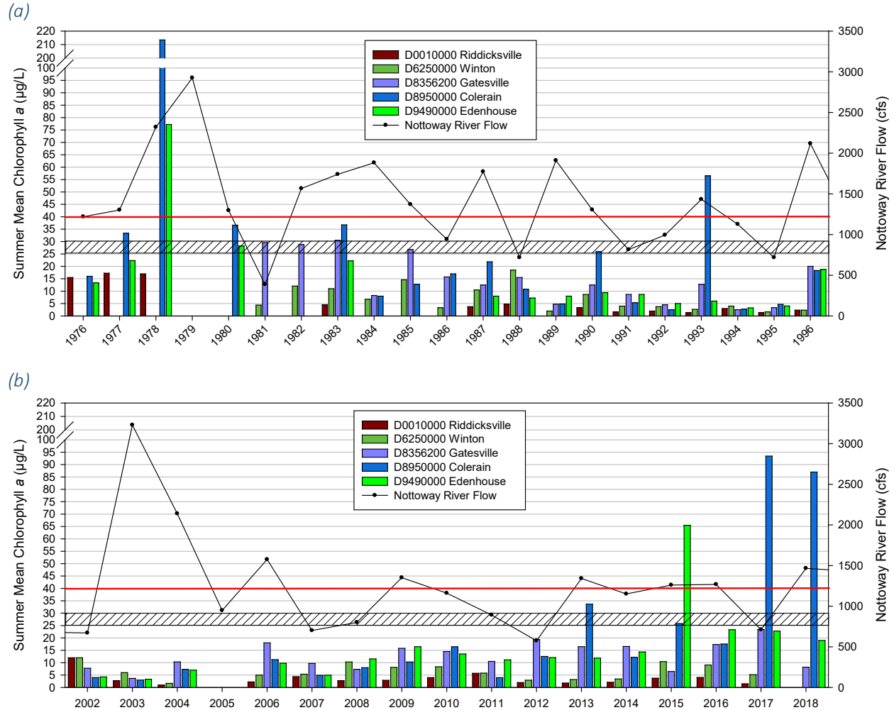
Figure 5-38: Chowan River Annual Mean Summer (June-September) Chlorophyll a Concentrations at the AMS Stations in the Basin (a) 1976-1996 and (b) 2002-2018. (Summer corresponds to the 1982 management plan goal of a target summer mean of no more than 25 to 30 \mu\text{g/L} Chlorophyll a (Hatched Zone); Red Line Indicates the 40 \mu\text{g/L} Chlorophyll a Standard; Note the Chlorophyll a Y-axis break needed to show the extreme 1978 concentration).
