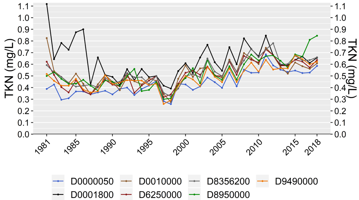
Figure 5-26: Annual Mean Total Kjeldahl Nitrogen Concentration (1981-2018) at (a) Two Virginia and Five Chowan River Mainstem AMS stations, (b) the Upper Three Station Only, (c) the Chowan River Station Only, and (d) Meherrin River Watershed Stations and the Chowan D6250000 at Winton.
