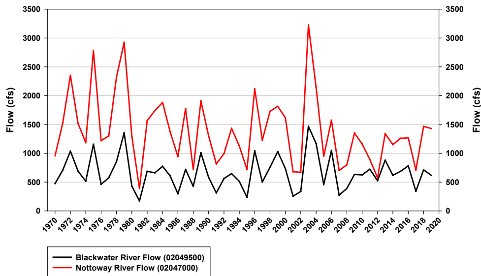
Figure 5-11: USGS Annual Stream Flow in the Nottoway and Blackwater rivers (1970-2019).
