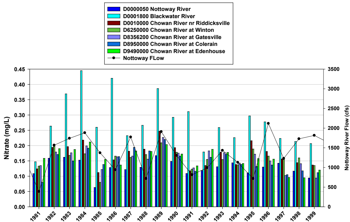
Figure 5-9: Annual Mean Nitrate Concentrations with Annual Nottoway River Flow (a) 1981-1999, (b) 2000-2018 and (c) 2006-2018 (This time frame focuses on the increase in the instream nitrate concentration over the last decade, note both Y-axis change to allow for better visual evaluation of the change that has occurred over this time period).
