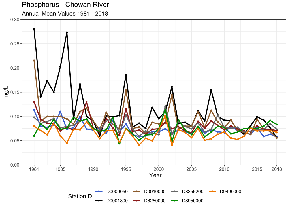
Figure 5-32: Annual Mean Total Phosphorus Concentration (1981-2018) at (a) Two Virginia and Five Chowan River Mainstem AMS stations, (b) the Upper Three Station Only, (c) the Chowan River Station Only, and (d) Meherrin River Watershed Stations and the Chowan D6250000 at Winton.
