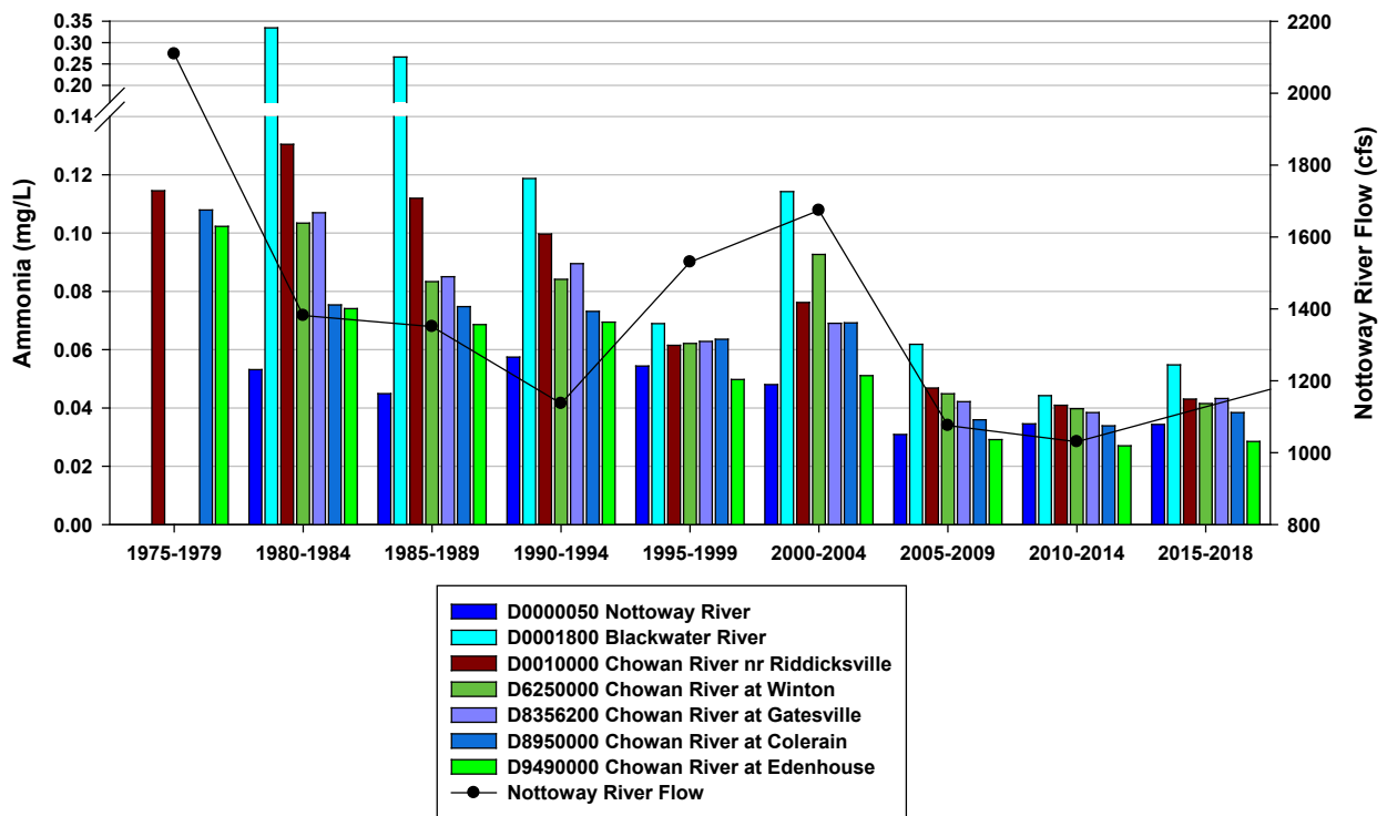
Figure 5-18: Five Year Mean Ammonia Concentrations and Nottoway River Flow (1975-2018). (Note the Y-axis scale break).
