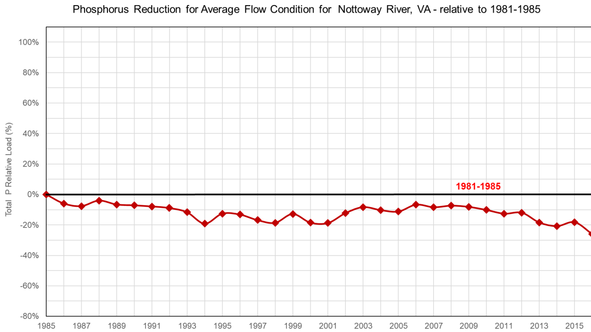
Figure 5-35: Flow-Normalized Total Phosphorus Load at (a) D0000050 Nottoway River, (b) D0001800 Blackwater River and (c) D4150000 Potecasi Creek Stations relative to the 1981-1985 Baseline Load.
