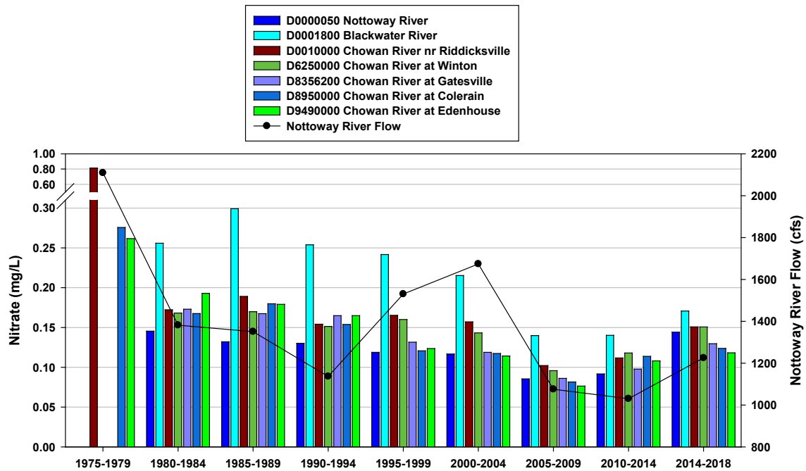
Figure 5-8: Five Year Mean Nitrate Concentrations and Nottoway River Flow (1975-2018).
