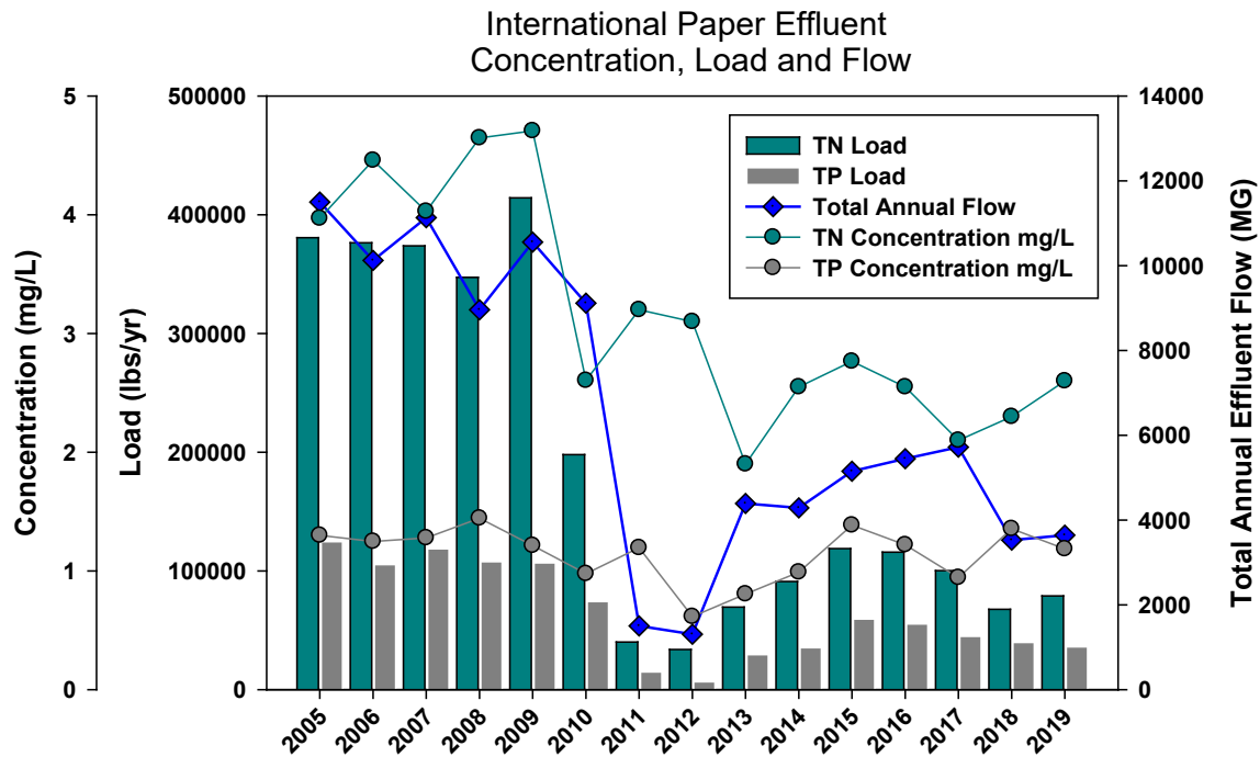
Figure 5-12: International Paper Winter Nutrient Effluent TN and TP Concentration, Load, and Total Annual Flow (Permitted Winter Season Discharge Flow Maximum of 14,000 MG).
