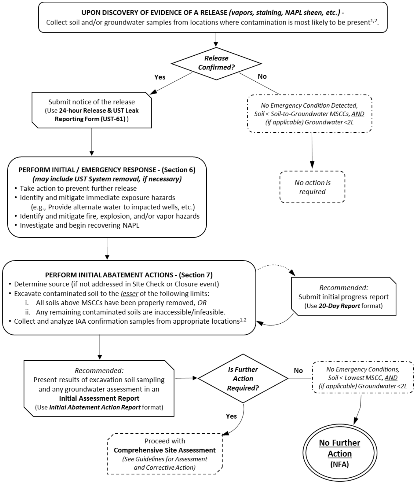
Figure 6 Flowchart of Requirements for NON-REGULATED NON-PETROLEUM UST Releases
