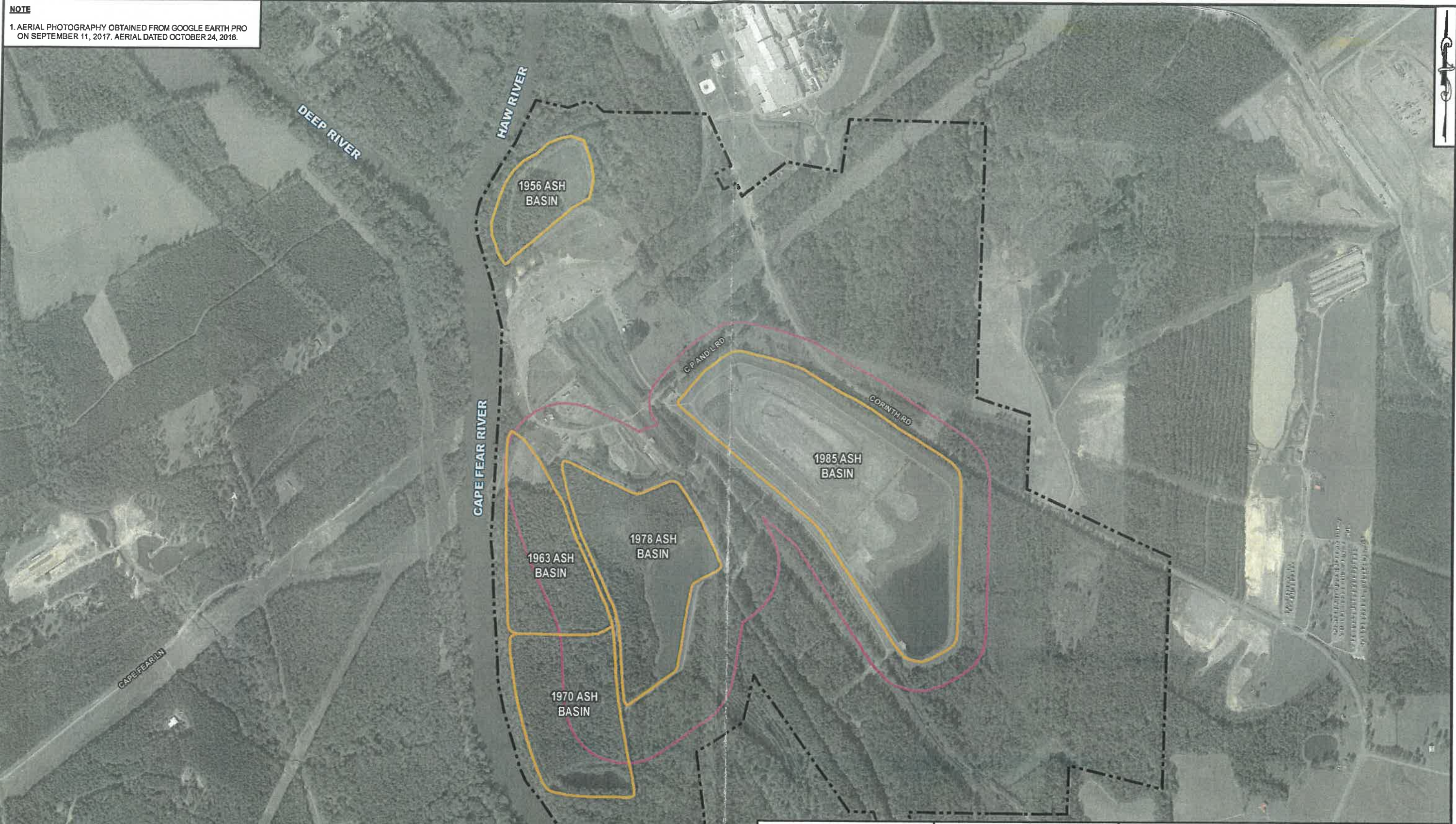
FIGURE 1 WASTE AND COMPLIANCE BOUNDARIES CAPE FEAR PLANT DUKE ENERGY PROGRESS, LLC MONCURE, NORTH CAROLINA
