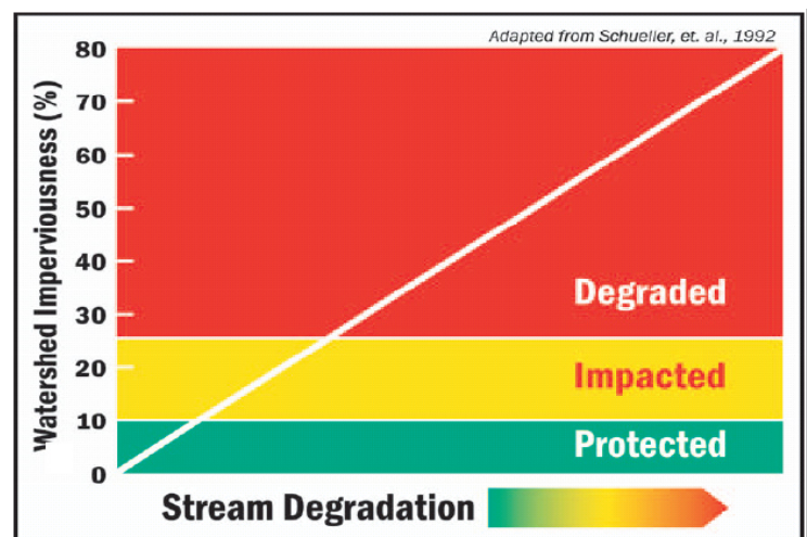
FIGURE 10-5: IMPERVIOUS COVER AND STREAM DEGRADATION
