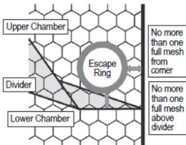
Figure 1: Placement of escape ring in crab pots with and without a divider (III.).
