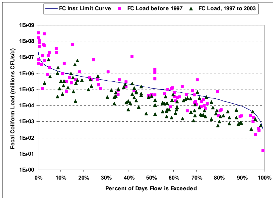
Figure 14. Instantaneous Fecal Coliform Load-Duration Curve (400/100 mL) for Chicod Creek at State Road 1760 Near Simpson, NC
