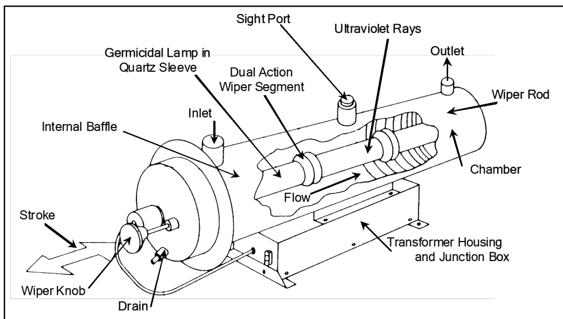
Figure 2-13. Ultraviolet radiation unit.
