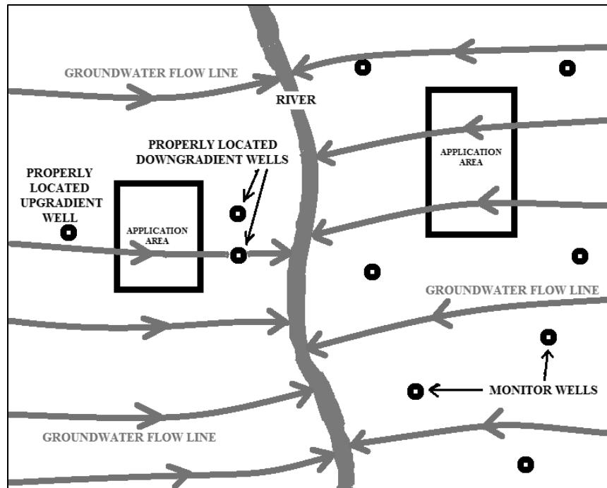
Figure 8-1. Proper well placement.
