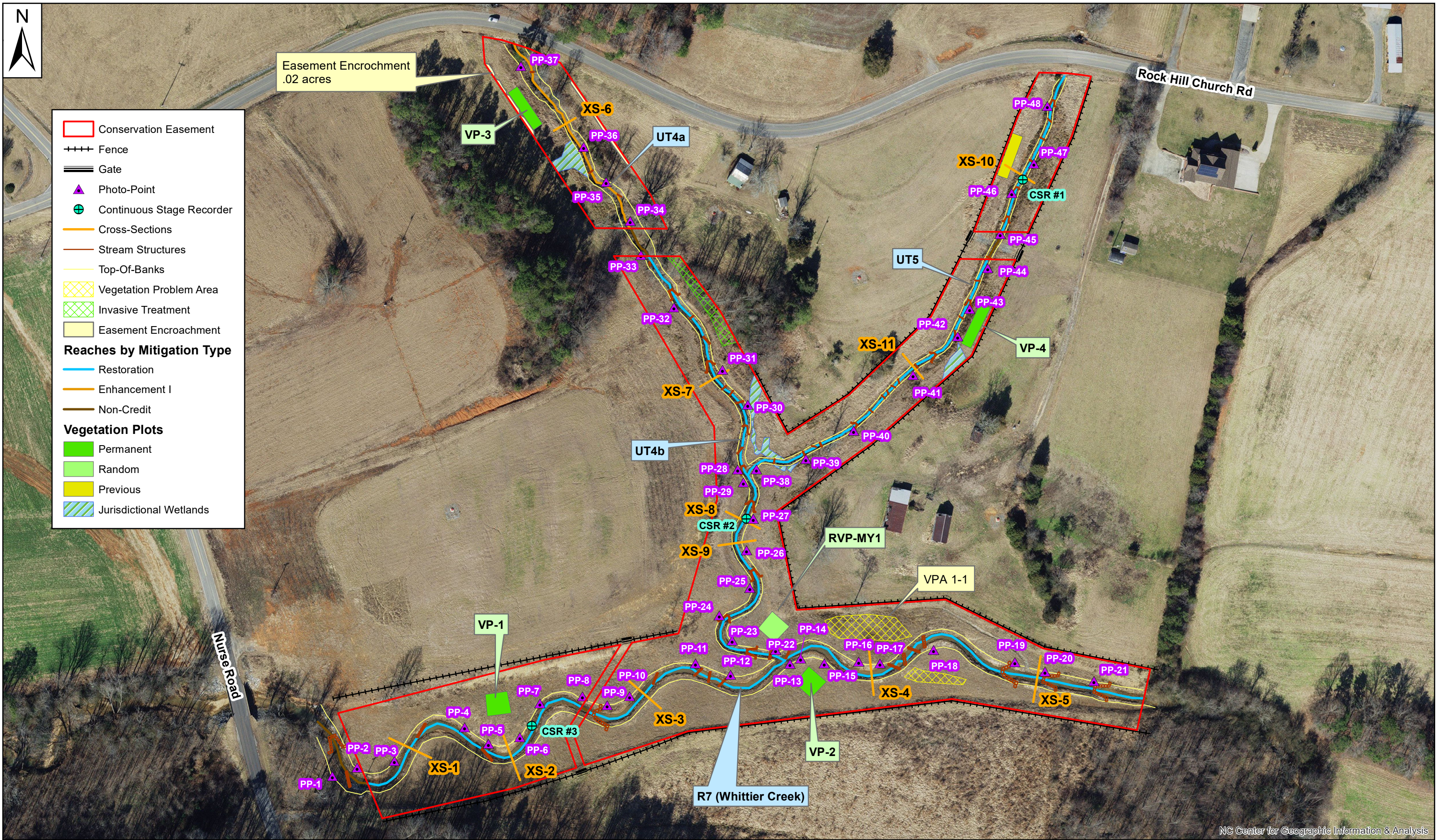
Figure 3. Current Conditions Plan View Monitoring Year 1 Whittier Creek Mitigation Project (#100020) Surry County, NC
